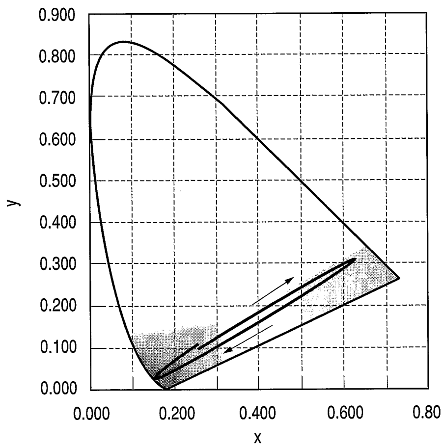
CHROMATICITY DIAGRAM
