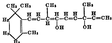
Compound XV
