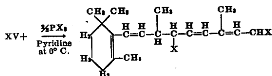
Compound XVI
