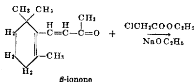
\beta -ionone
