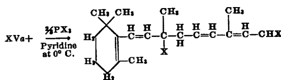
Compound XVIa
