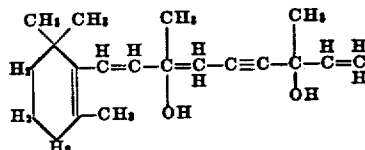
Compound XIVa
