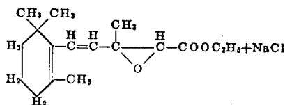
Compound II
