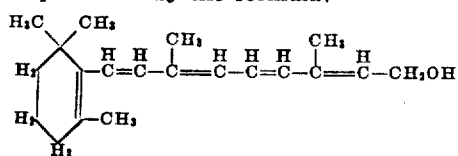
Compound I
