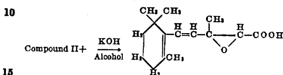
Compound III
