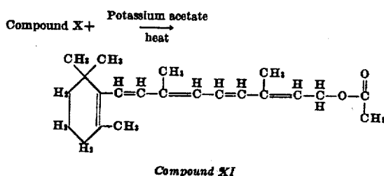
Compound XI
