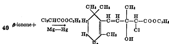
Compound IIa
