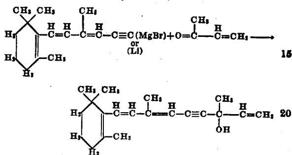
Compound VIII
