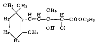
Compound IIa
