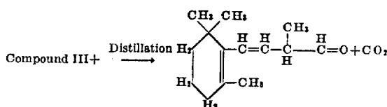
Compound IV
