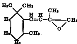
Compound IVa
