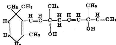
Compound XVa
