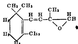
Compound IVa
