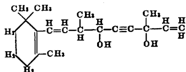
Compound XIV
