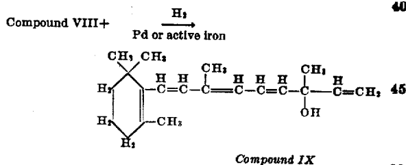
Compound IX
