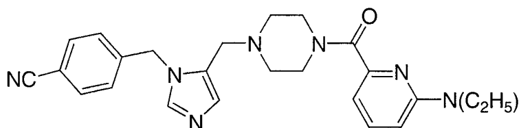
4-[1-(4-Cyanobenzyl)imidazol-5-ylmethyl]-1-(6-diethylamino-pyrid-2-yl)piperazine
