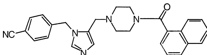
4-[1-(4-Cyanobenzyl)imidazol-5-ylmethyl]-1-(1-naphthoyl)piperazine
