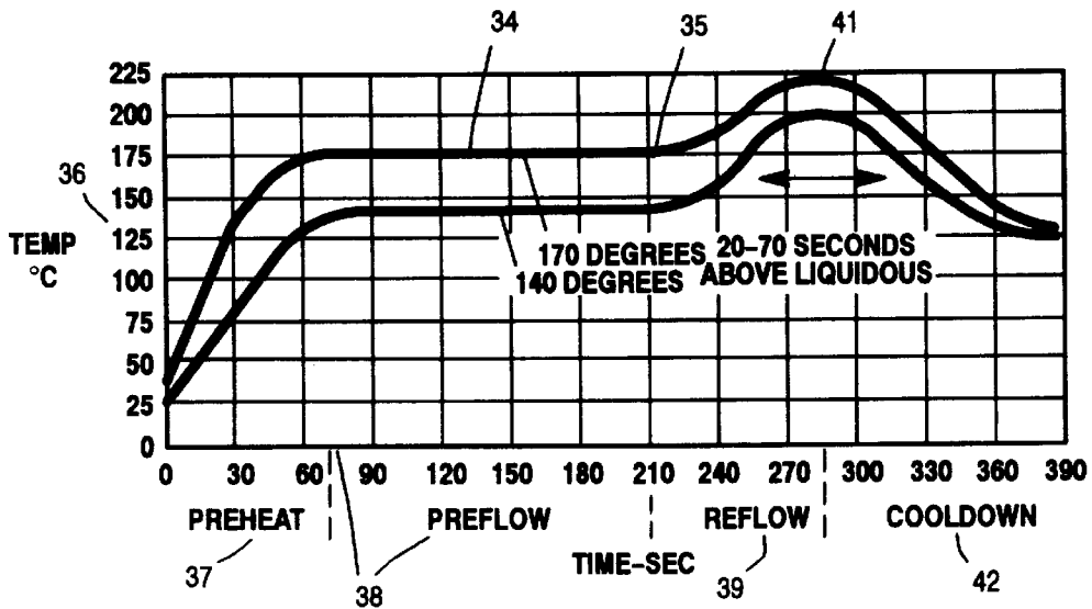
Figure 3 Prior Art
