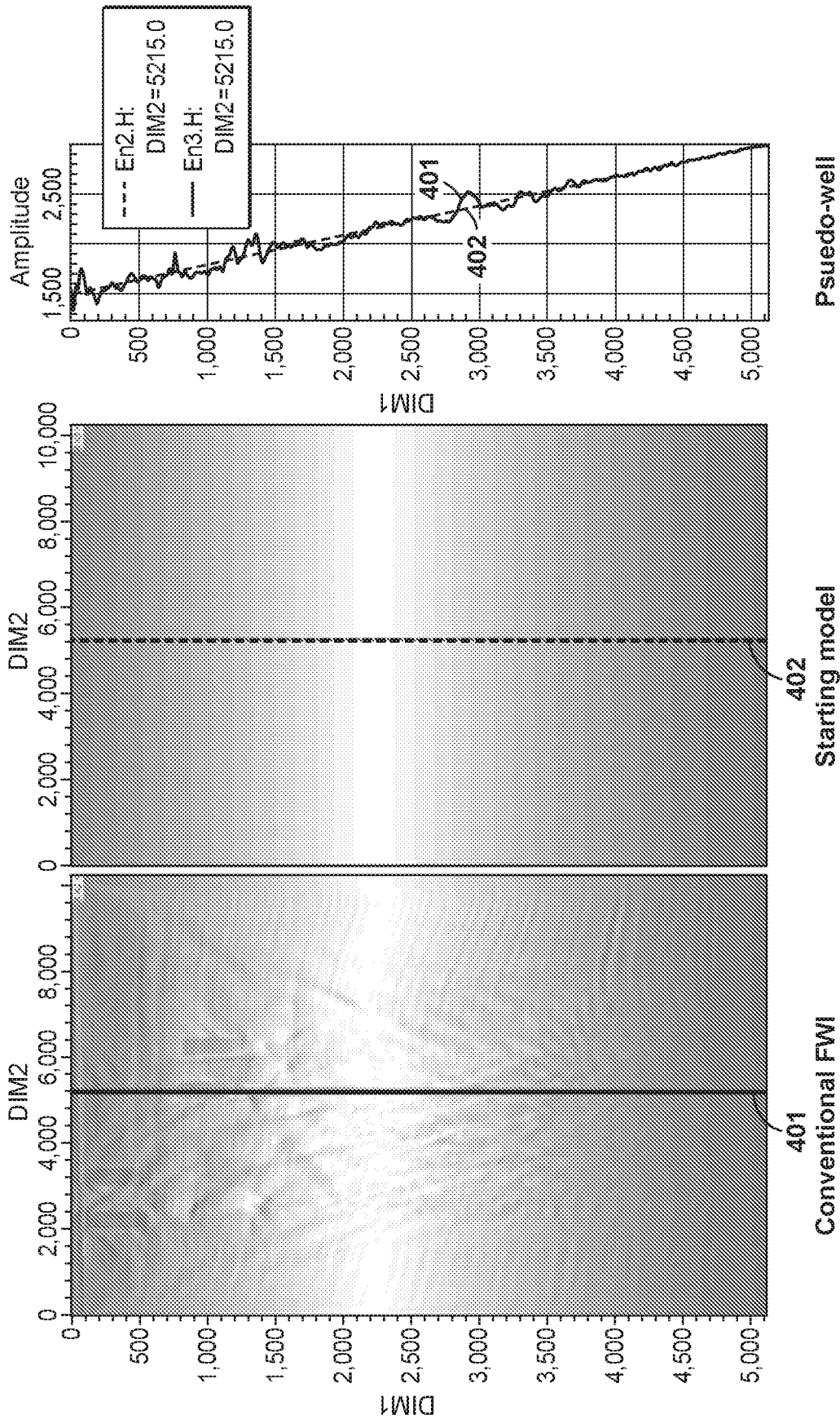
Standard FWI Result: Inverted Vp Model and Starting Model
