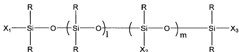
General Formula (1)
