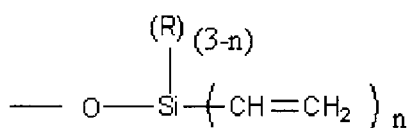
Substituent A
