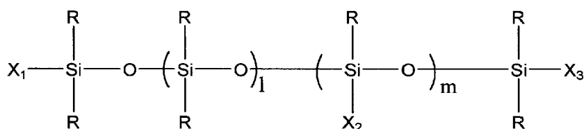
General Formula (1)
