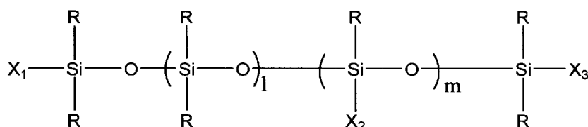
General Formula (1)
