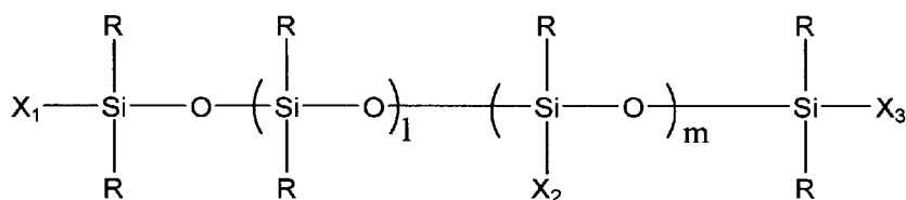
General Formula (1)
