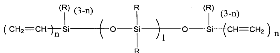
General Formula (2)
