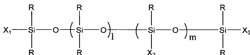
General Formula (1)
