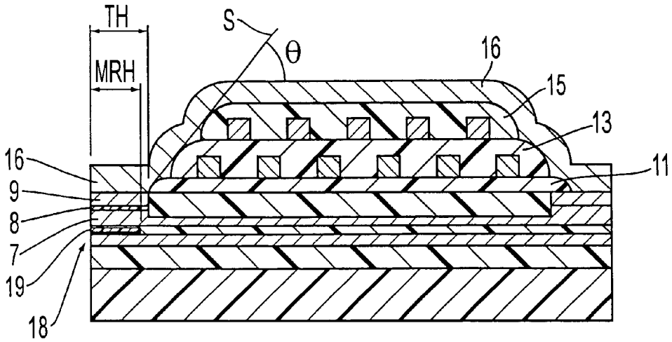
FIG. 10 PRIOR ART
