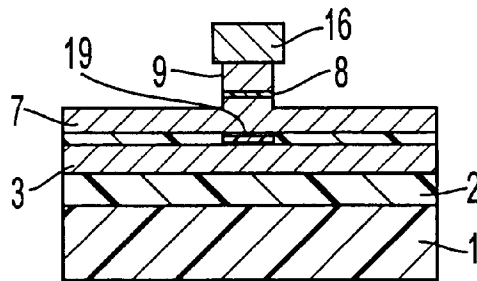
FIG. 11 PRIOR ART
