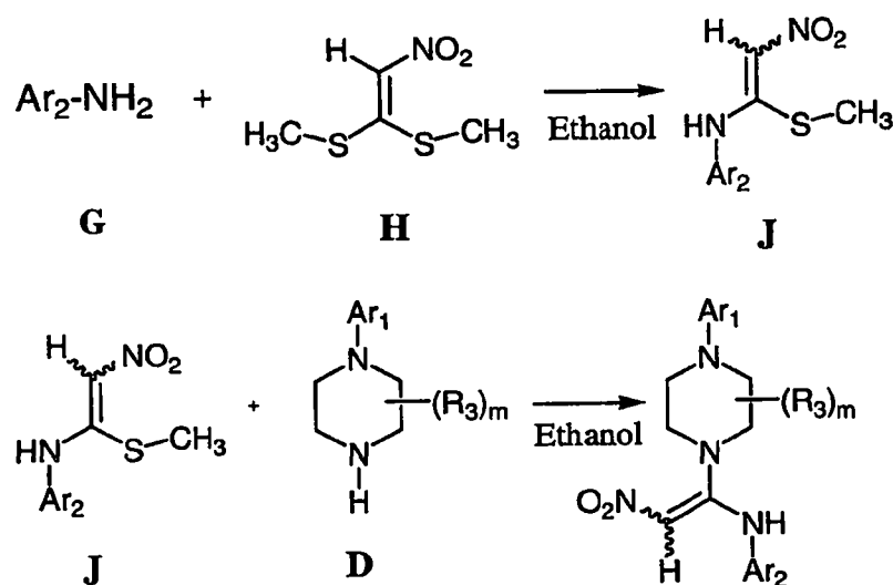
Cyano(nitro)vinylpiperazine Compound of Formula (II)
