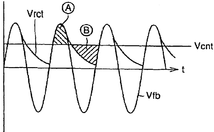
FIG. 9A FOR SMALL RECTIFICATION TIME-CONSTANT PRIOR ART
