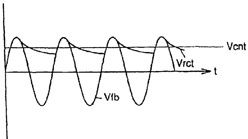
FIG. 9B FOR LARGE RECTIFICATION TIME-CONSTANT PRIOR ART
