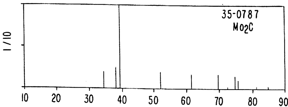
REFERENCE XRD PATTERN, HEXAGONAL Mo 2 C
