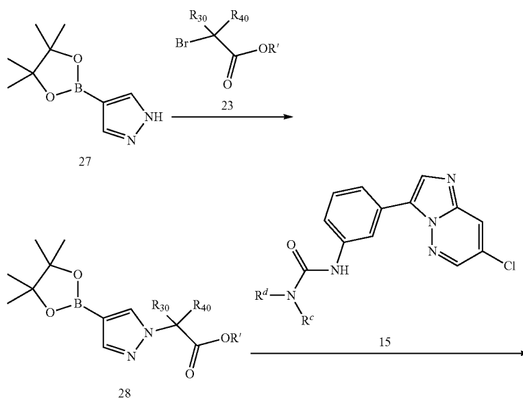
Scheme 7
