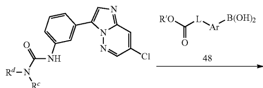
Scheme 13
