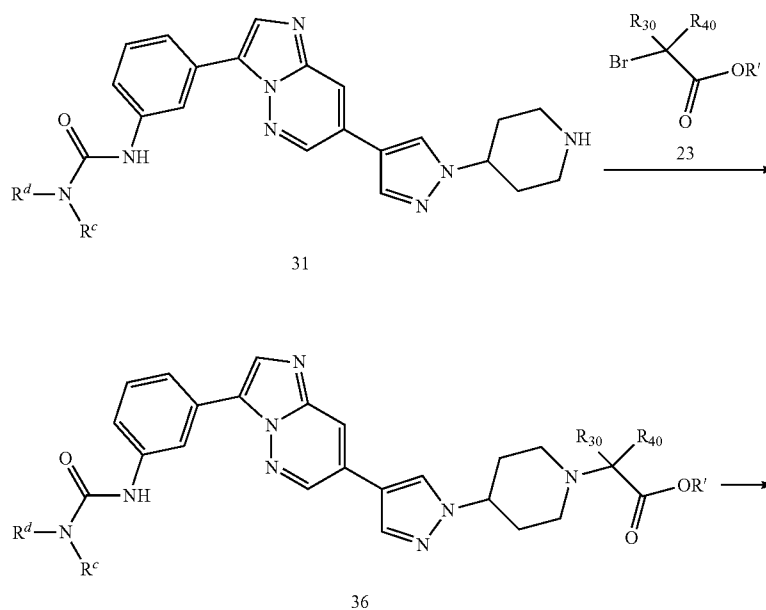
Scheme 10
