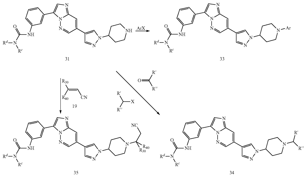
Scheme 9
