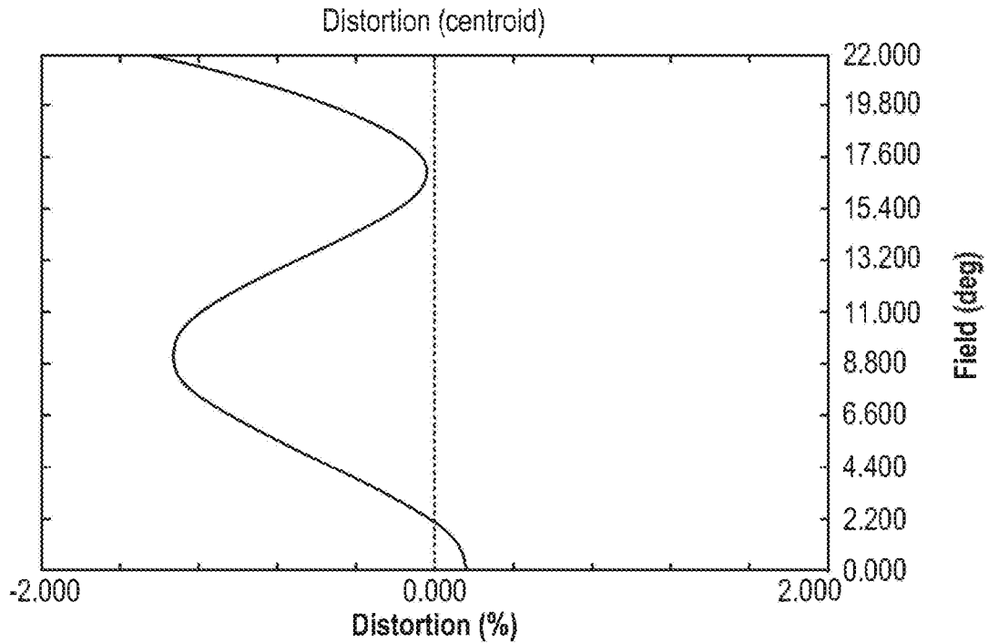
30/06/2013 Maximum distortion = 1.5%
