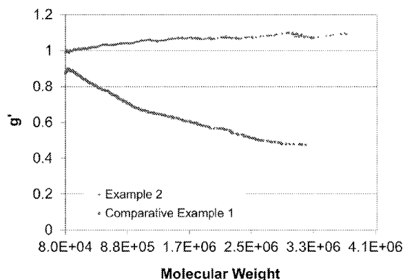
g' Long Chain Branching of Polypropylene Resin
