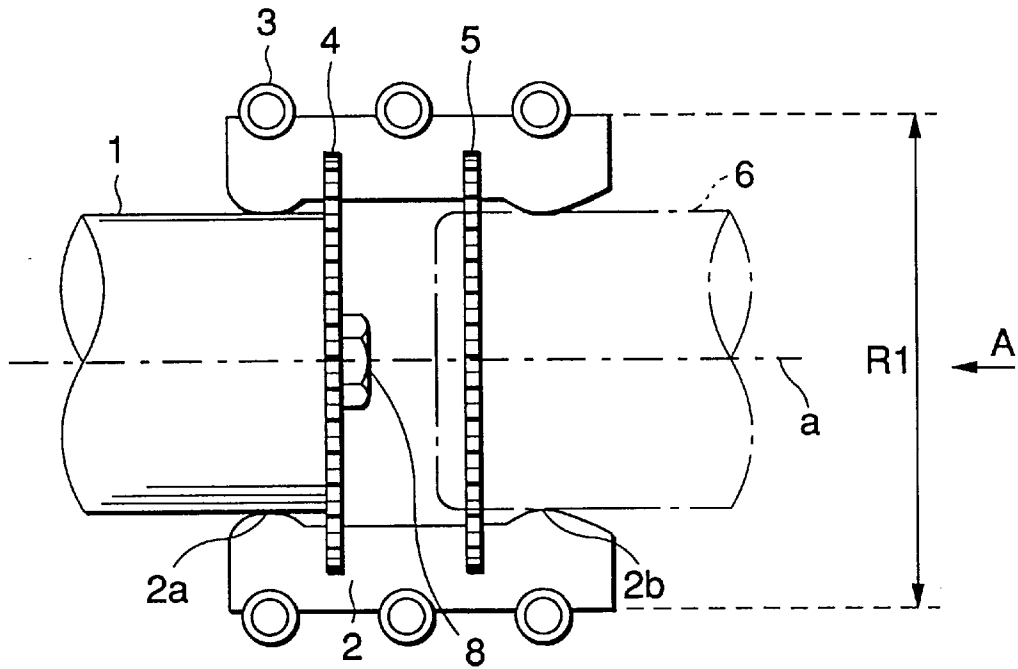
FIG.7 PRIOR ART
