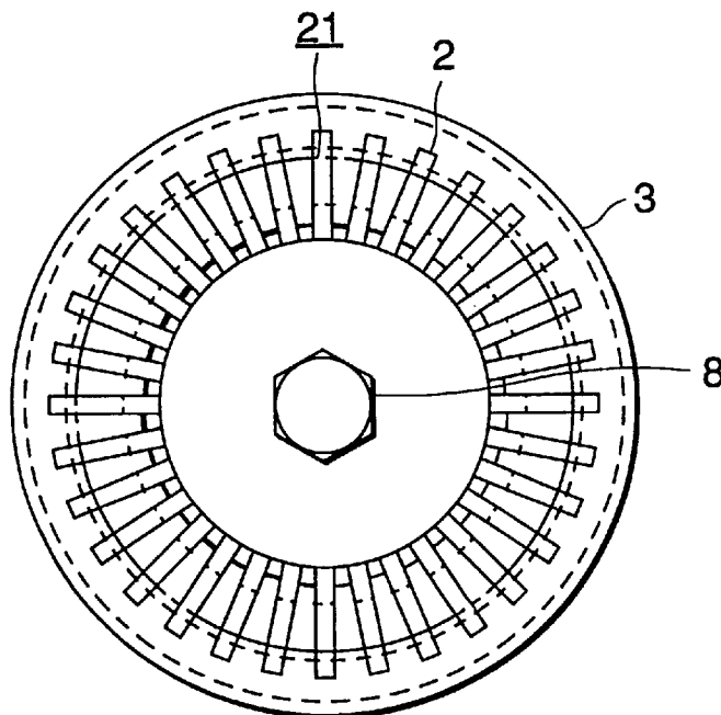
FIG.8 PRIOR ART
