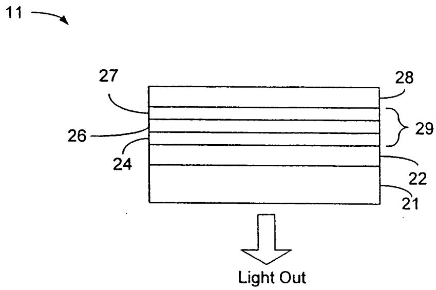
Fig. 1 (Prior Art)
