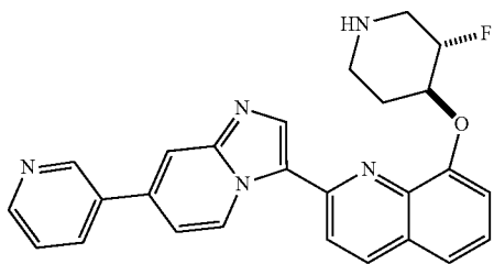
8-((trans)-3-fluoropiperidin-4-yloxy)-2-(7-(pyridin-3-yl)imidazo[1,2-a]pyridin-3-yl)quinoline
