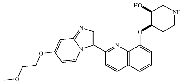
(cis)-4-(2-(7-(2-methoxyethoxy)imidazo[1,2-a]pyridin-3-yl)quinolin-8-yloxy)piperidin-3-ol
