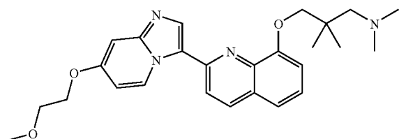
3-(2-(7-(2-methoxyethoxy)imidazo[1,2-a]pyridin-3-yl)quinolin-8-yloxy)-N,N,2,2-tetramethylpropan-1-amine
