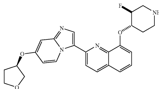
8-((trans)-3-fluoropiperidin-4-yloxy)-2-(7-((R)-tetrahydrofuran-3-yloxy)imidazo[1,2-a]pyridin-3-yl)quinoline
