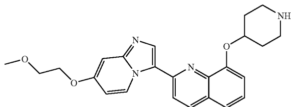
2-(7-(2-methoxyethoxy)imidazo[1,2-a]pyridin-3-yl)-8-(piperidin-4-yloxy)quinoline
