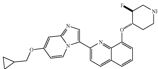
2-(7-(cyclopropylmethoxy)imidazo[1,2-a]pyridin-3-yl)-8-((trans)-3-fluoropiperidin-4-yloxy)quinoline
