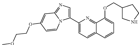
2-(7-(2-methoxyethoxy)imidazo[1,2-a]pyridin-3-yl)-8-(pyrrolidin-3-ylmethoxy)quinoline
