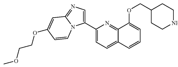
2-(7-(2-methoxyethoxy)imidazo[1,2-a]pyridin-3-yl)-8-(piperidin-4-ylmethoxy)quinoline
