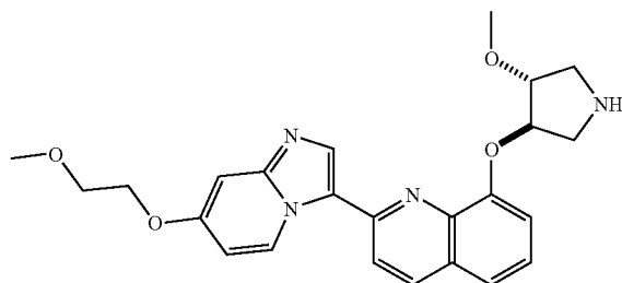
2-(7-(2-methoxyethoxy)imidazo[1,2-a]pyridin-3-yl)- 8-((trans)-4-methoxypyrrolidin-3-yloxy)quinoline
