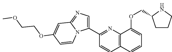
(R)-2-(7-(2-methoxyethoxy)imidazo[1,2-a]pyridin-3-yl)-8-(pyrrolidin-2-ylmethoxy)quinoline
