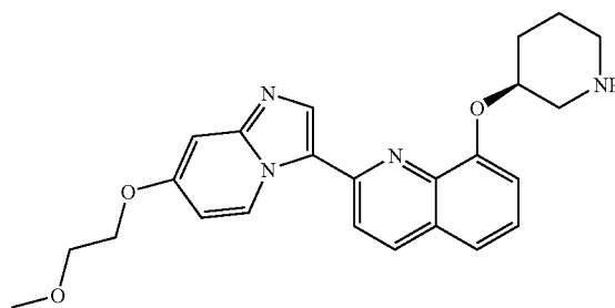
(S)-2-(7-(2-methoxyethoxy)imidazo[1,2-a]pyridin-3-yl)-8-(piperidin-3-yloxy)quinoline
