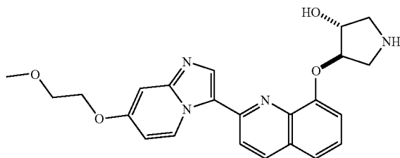
(trans)-4-(2-(7-(2-methoxyethoxy)imidazo[1,2-a]pyridin-3-yl)quinolin-8-yloxy)pyrrolidin-3-ol
