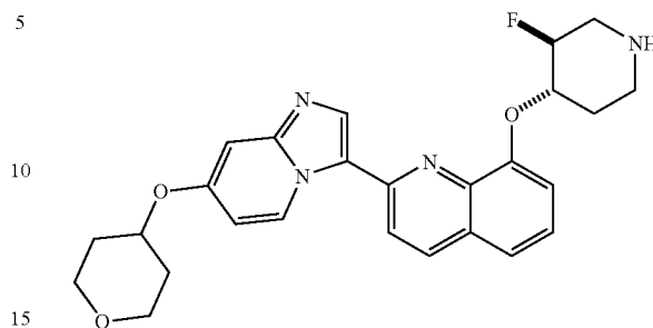
8-((trans)-3-fluoropiperidin-4-yloxy)-2-(7-(tetrahydro-2H-pyran-4-yloxy)imidazo[1,2-a]pyridin-3-yl)quinoline
