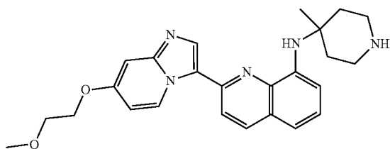
2-(7-(2-methoxyethoxy)imidazo[1,2-a]pyridin-3-yl)- N-(4-methylpiperidin-4-yl)quinolin-8-amine
