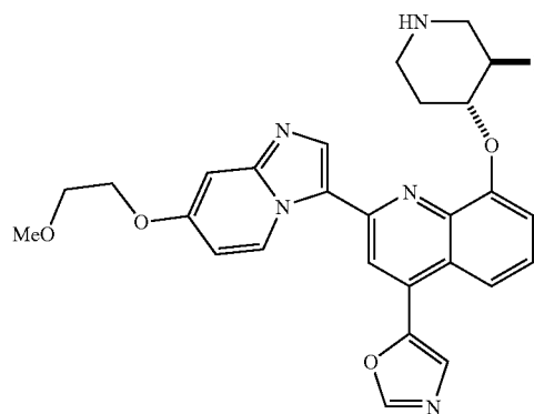
5-(8-((trans)-3-fluoropiperidin-4-yloxy)-2-(7-(2-methoxyethoxy)imidazo[1,2-a]pyridin-3-yl)quinolin-4-yl)oxazole
