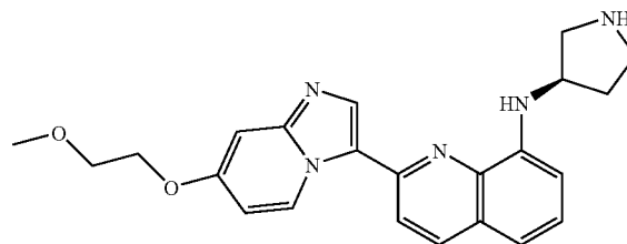
(R)-2-(7-(2-methoxyethoxy)imidazo[1,2-a]pyridin-3-yl)-N-(pyrrolidin-3-yl)quinolin-8-amine
