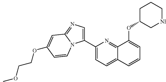
(R)-2-(7-(2-methoxyethoxy)imidazo[1,2-a]pyridin-3-yl)-8-(piperidin-3-yloxy)quinoline
