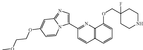
8-((4-fluoropiperidin-4-yl)methoxy)-2-(7-(2-methoxyethoxy)imidazo[1,2-a]pyridin-3-yl)quinoline
