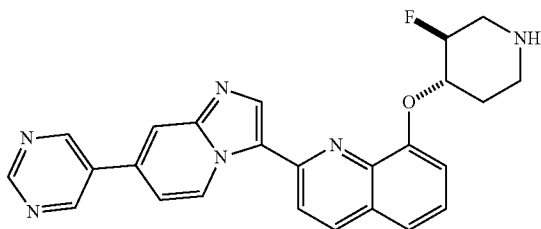
8-((trans)-3-fluoropiperidin-4-yloxy)-2-(7-(pyrimidin-5-yl)imidazo[1,2-a]pyridin-3-yl)quinoline
