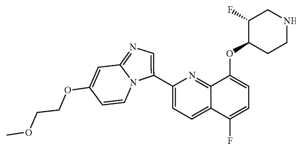
5-fluoro-8-((3R,4R)-3-fluoropiperidin-4-yloxy)-2-(7-(2-methoxyethoxy)imidazo[1,2-a]pyridin-3-yl)quinoline
