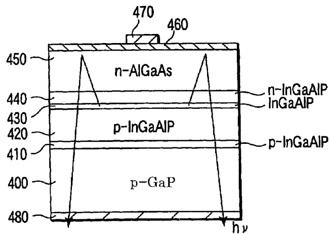
FIG. 5 PRIOR ART
