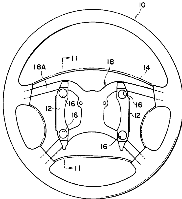
FIG. 10 PRIOR ART
