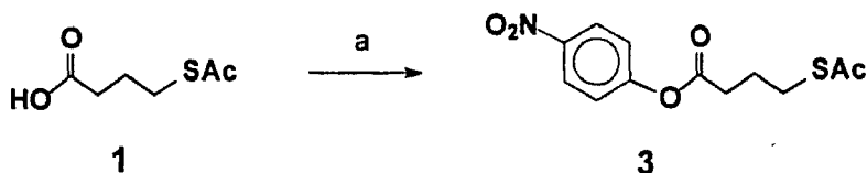
Scheme 2. Synthesis of the linking reagent 3. a: CF 3 COOpNp, Et 3 N.
