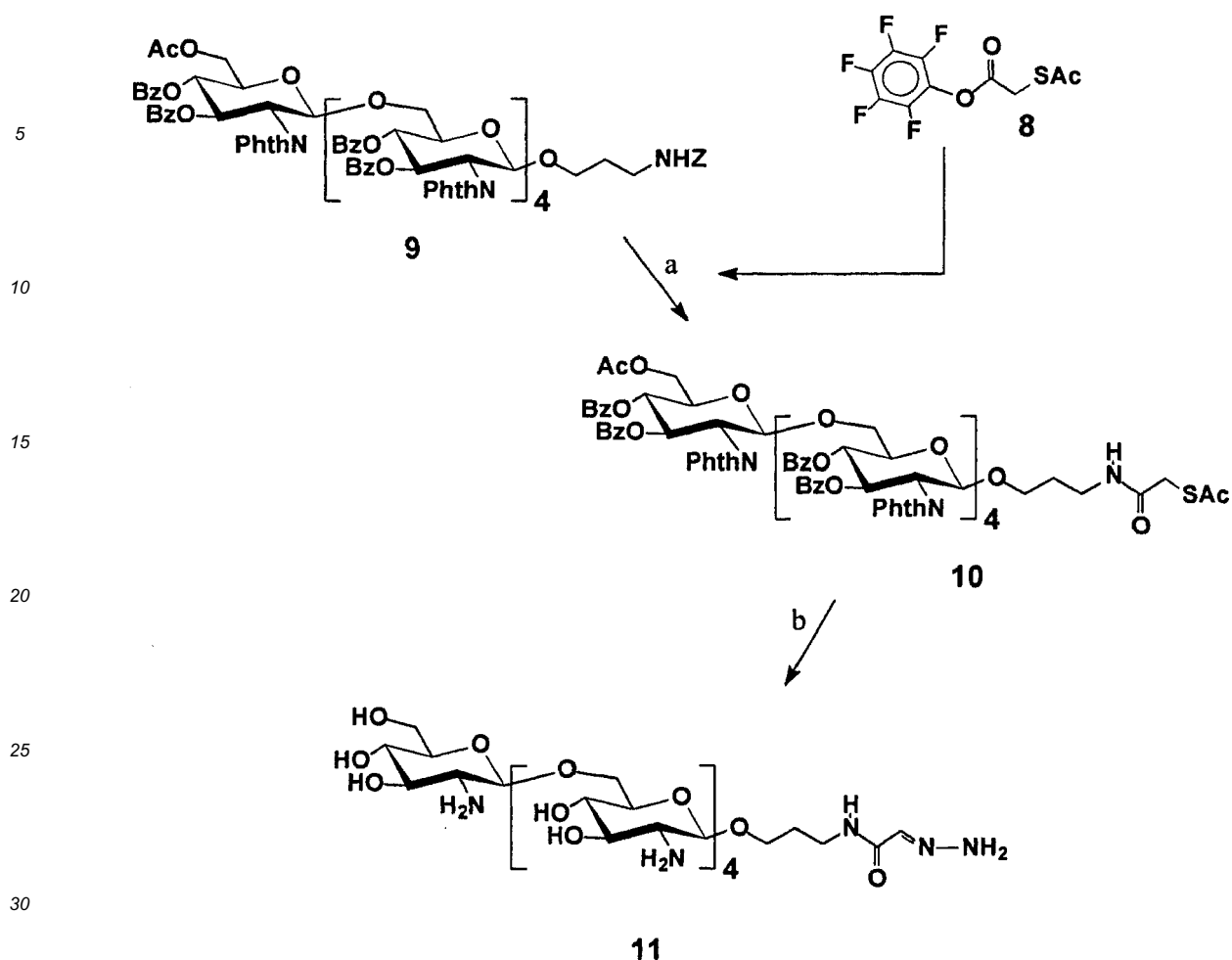
Scheme 4. Synthesis of the ligands.. a: 1) \text{H}_2 , \text{Pd}(\text{OH})_2/\text{C} , \text{MeOH}/\text{THF} 2) 8 , \text{Et}_3\text{N} , \text{CH}_2\text{Cl}_2 ; b: \text{N}_2\text{H}_4 \cdot \text{H}_2\text{O} , \text{EtOH} , \Delta .
