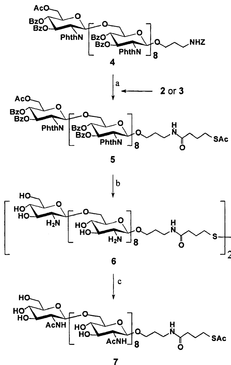
Scheme 3. Synthesis of the ligands. a: 1) \text{H}_2 , \text{Pd}(\text{OH})_2/\text{C} , \text{MeOH}/\text{THF} 2) 2 or 3, \text{Et}_3\text{N} , \text{CH}_2\text{Cl}_2 ; b: \text{N}_2\text{H}_4 \cdot \text{H}_2\text{O} , \text{EtOH} , \Delta ; c: DTT, \text{NaHCO}_3 , \text{Ac}_2\text{O} , \text{MeOH}/\text{H}_2\text{O} .
