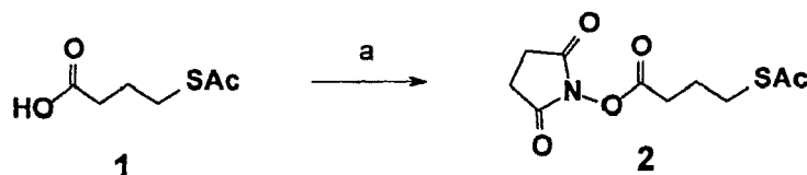
Scheme 1. Synthesis of the linking reagent 2. a: CF 3 COOSu, pyridine.
