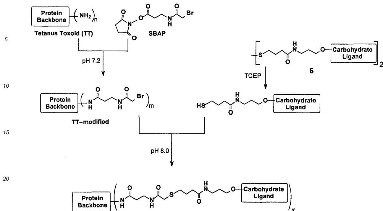
Conjugate of Tetanus Toxoid with Ligand 6 ("TT-9NH 2 ")
