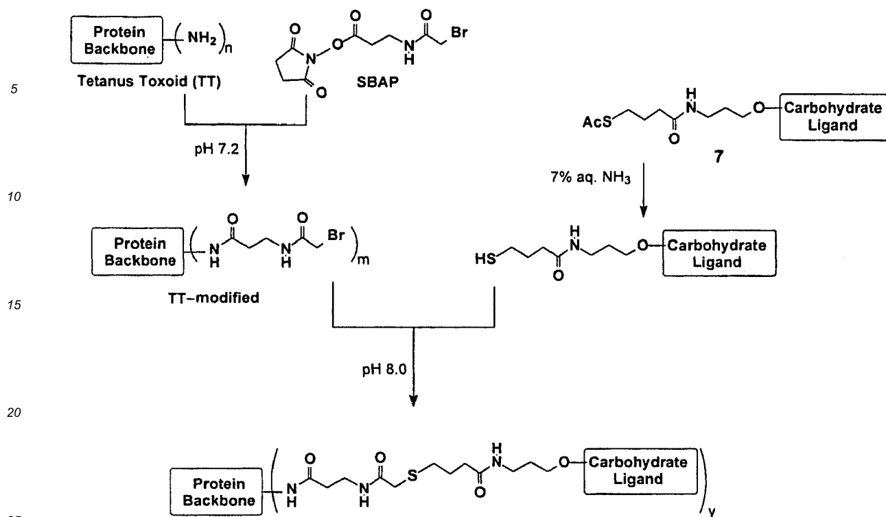
Conjugate of Tetanus Toxoid with Ligand 7 ("TT-9NAC")
