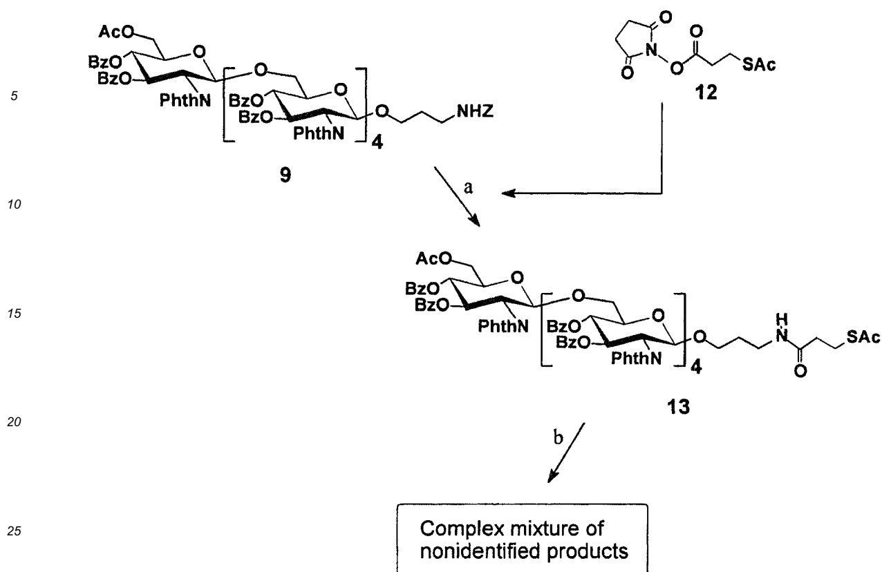
Scheme 5. Synthesis of the ligands.. a: 1) \text{H}_2 , \text{Pd}(\text{OH})_2/\text{C} , \text{MeOH}/\text{THF} 2) 12 , \text{Et}_3\text{N} , \text{CH}_2\text{Cl}_2 ; b: \text{N}_2\text{H}_4 \cdot \text{H}_2\text{O} , \text{EtOH} , \Delta
