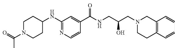
Compound 254
