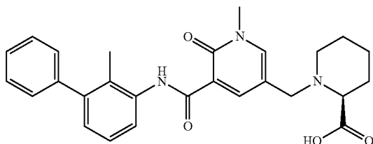
Step 1: 2-methylbiphenyl-3-amine
