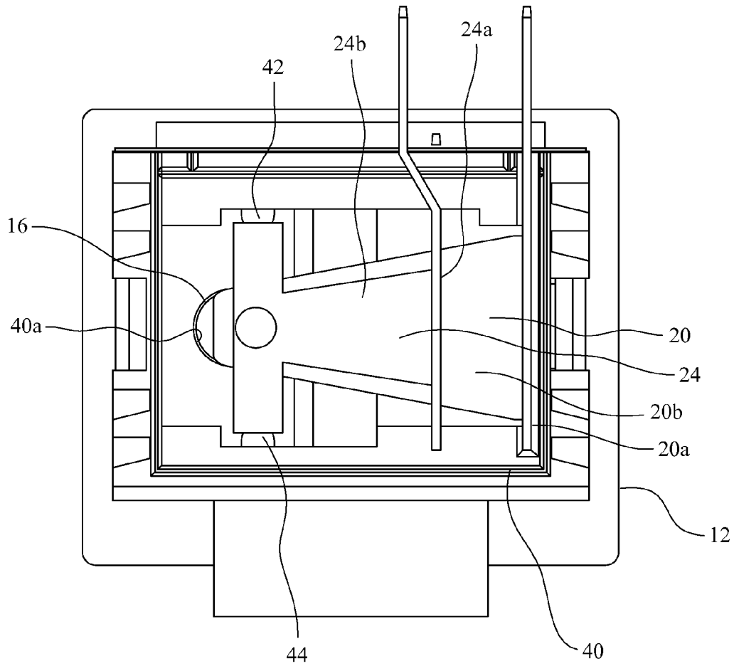
FIG. 7 (BOTTOM VIEW)
