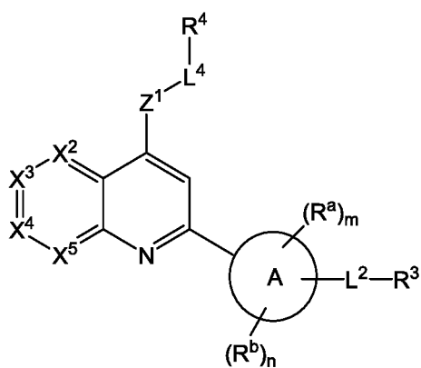
Formula (II).
