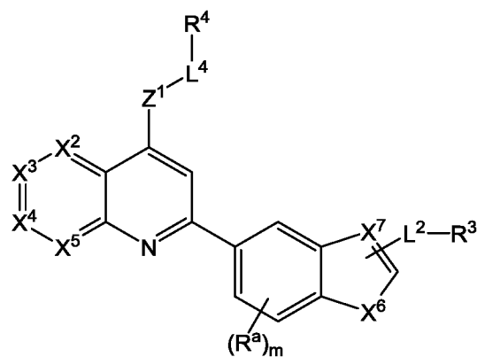
Formula (IV)
