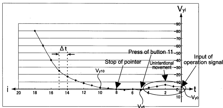
History of displacement corresponding amount V_{yi} stored in memory
