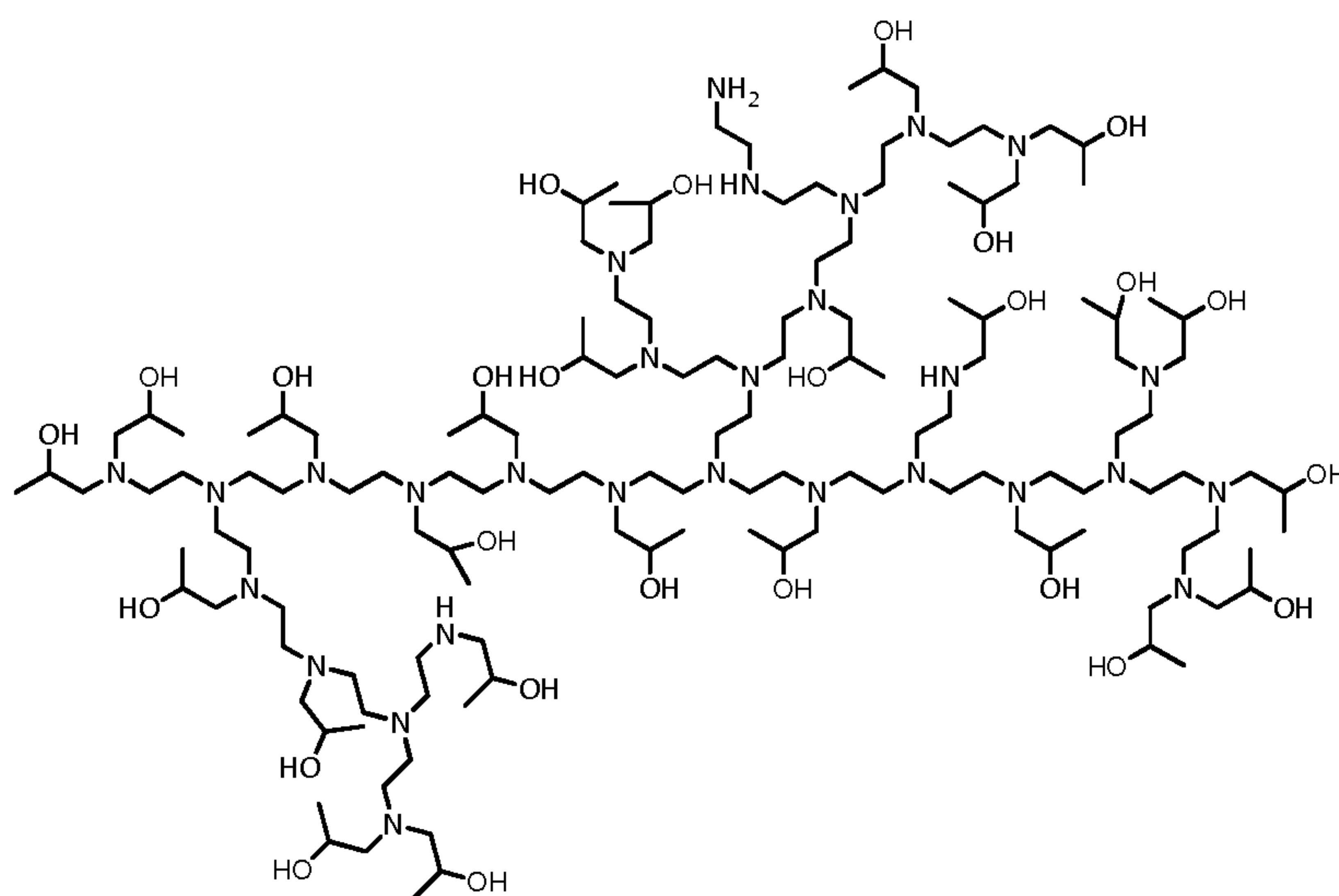
(structure 2)
