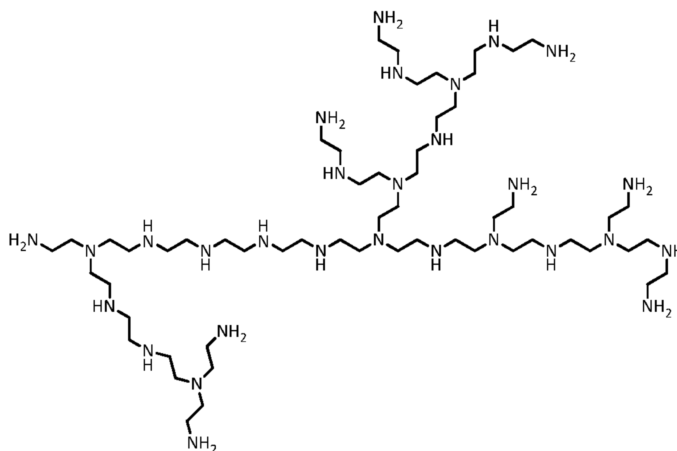
(structure 1)
