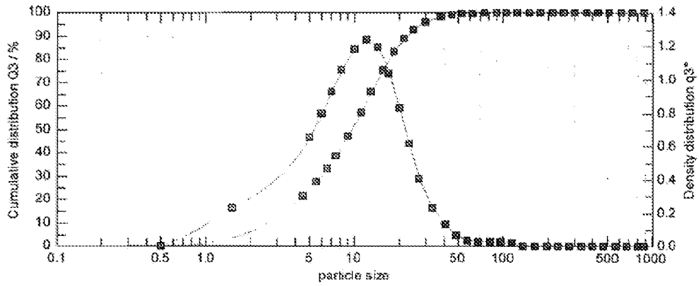
cumulative distribution
