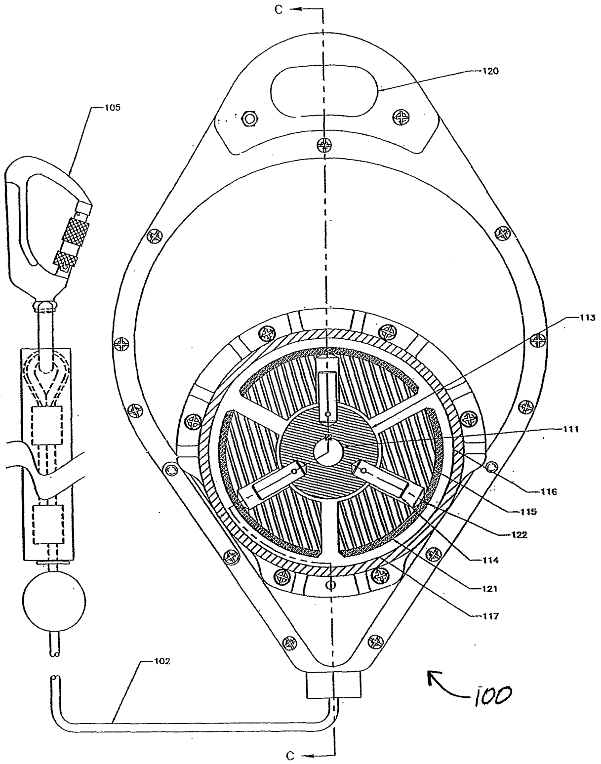
FIG. 1 PRIOR ART
