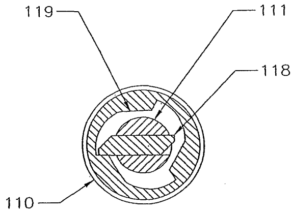
FIG. 3 PRIOR ART
