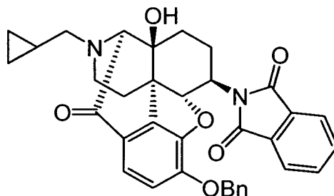
Compound 6
