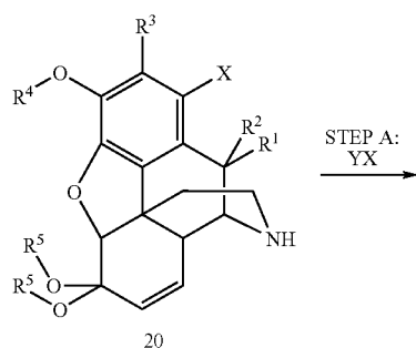
Reaction Scheme 2:
