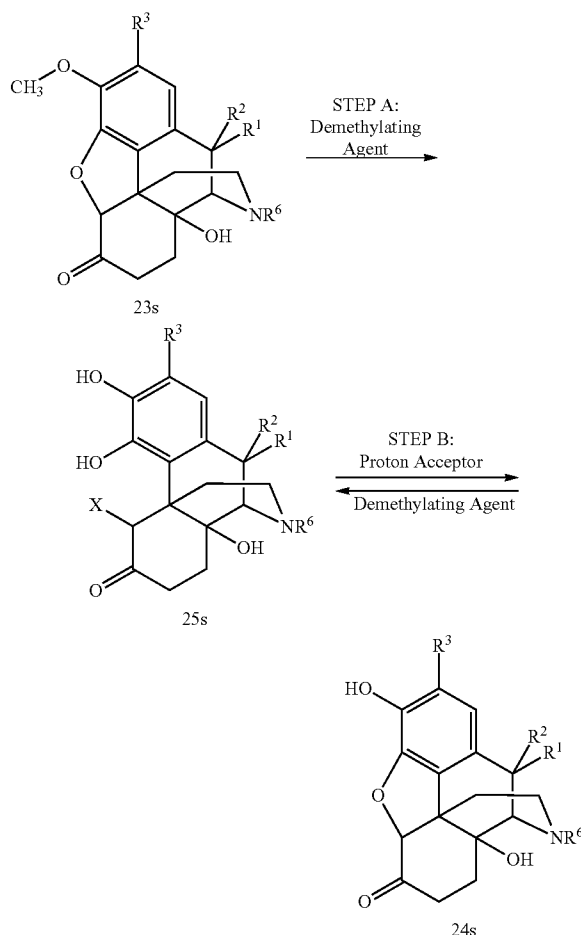
Reaction Scheme 3:
