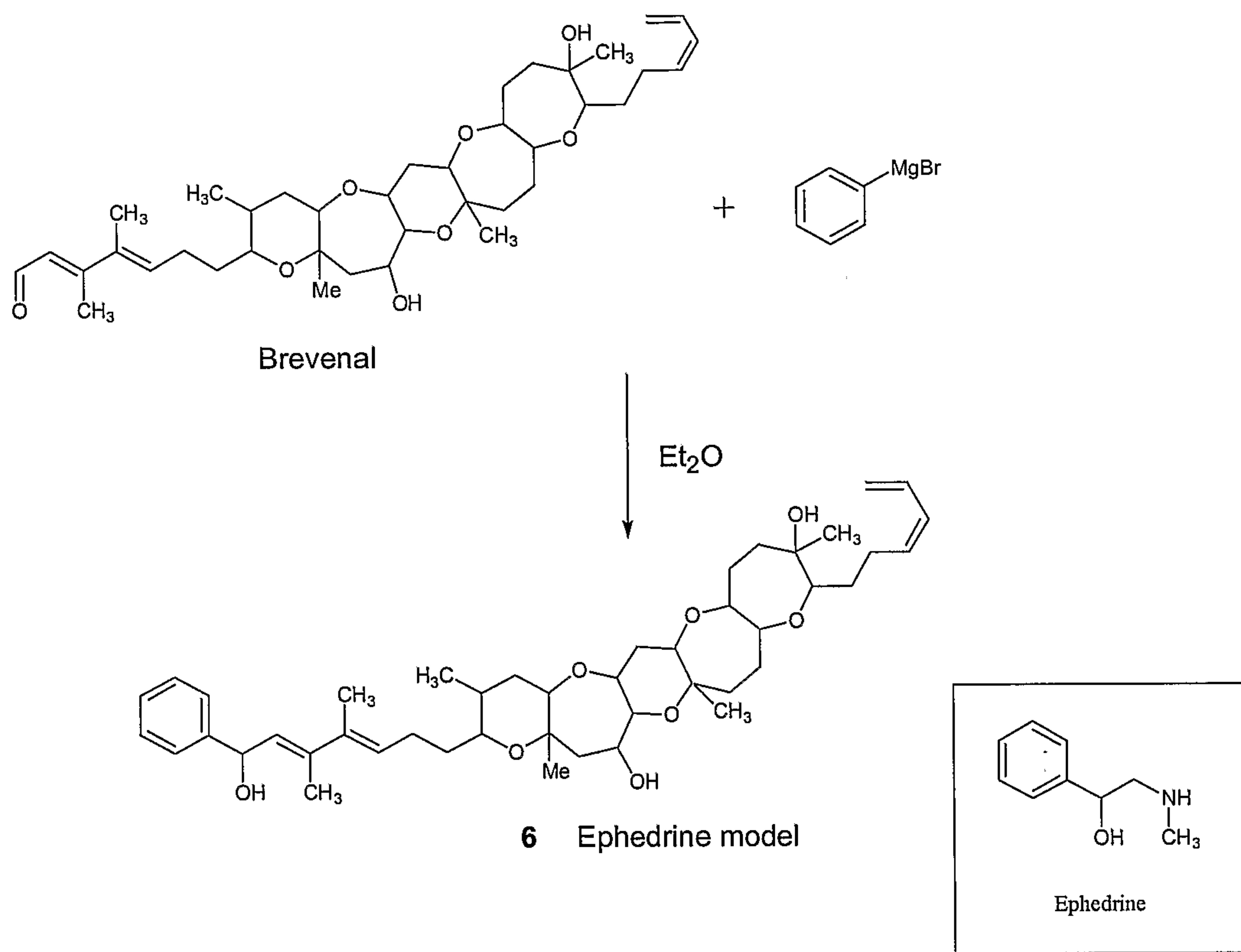
Scheme 4: Synthesis of an ephedrine model of brevenal
