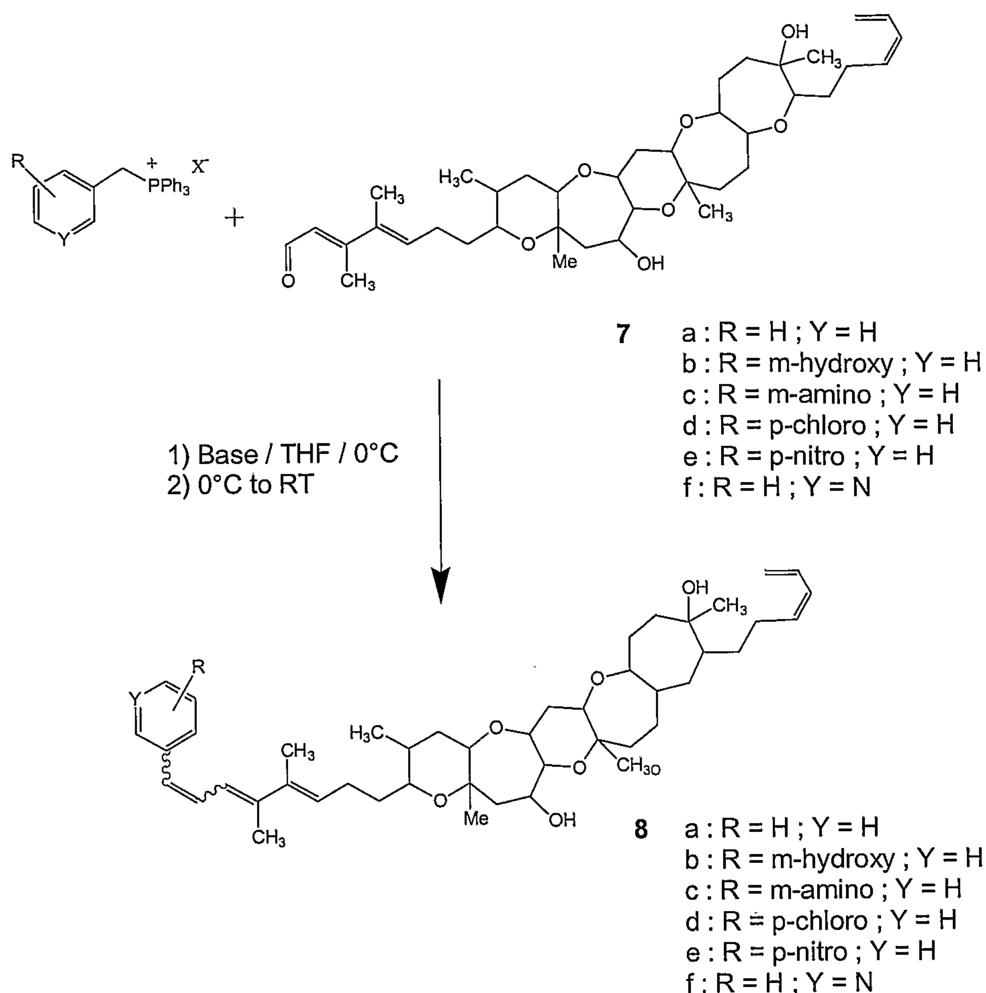
Scheme 5: Synthesis of benzenic derivatives
