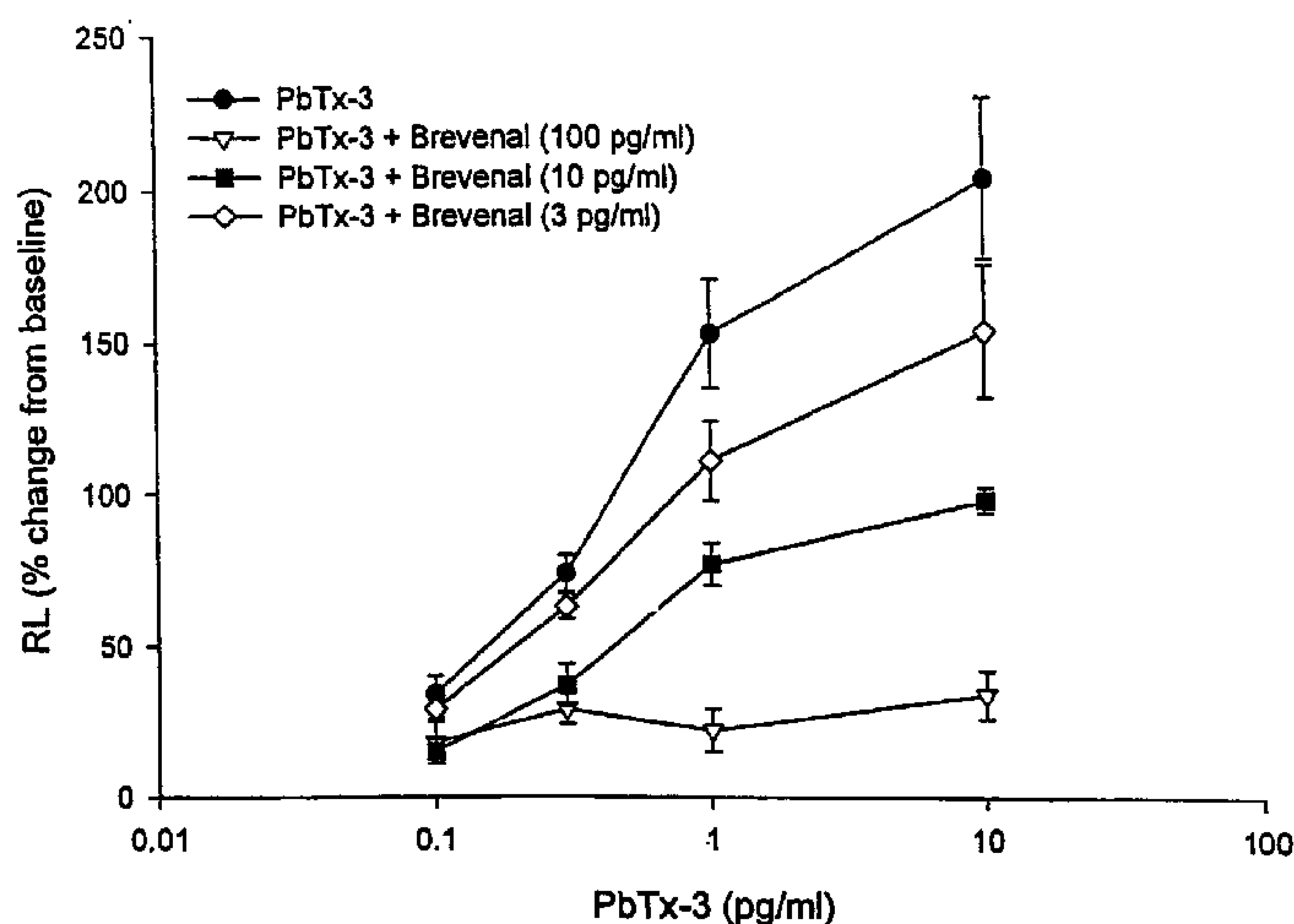
Effect of Brevenal on PbTx-3 Induced Constriction
