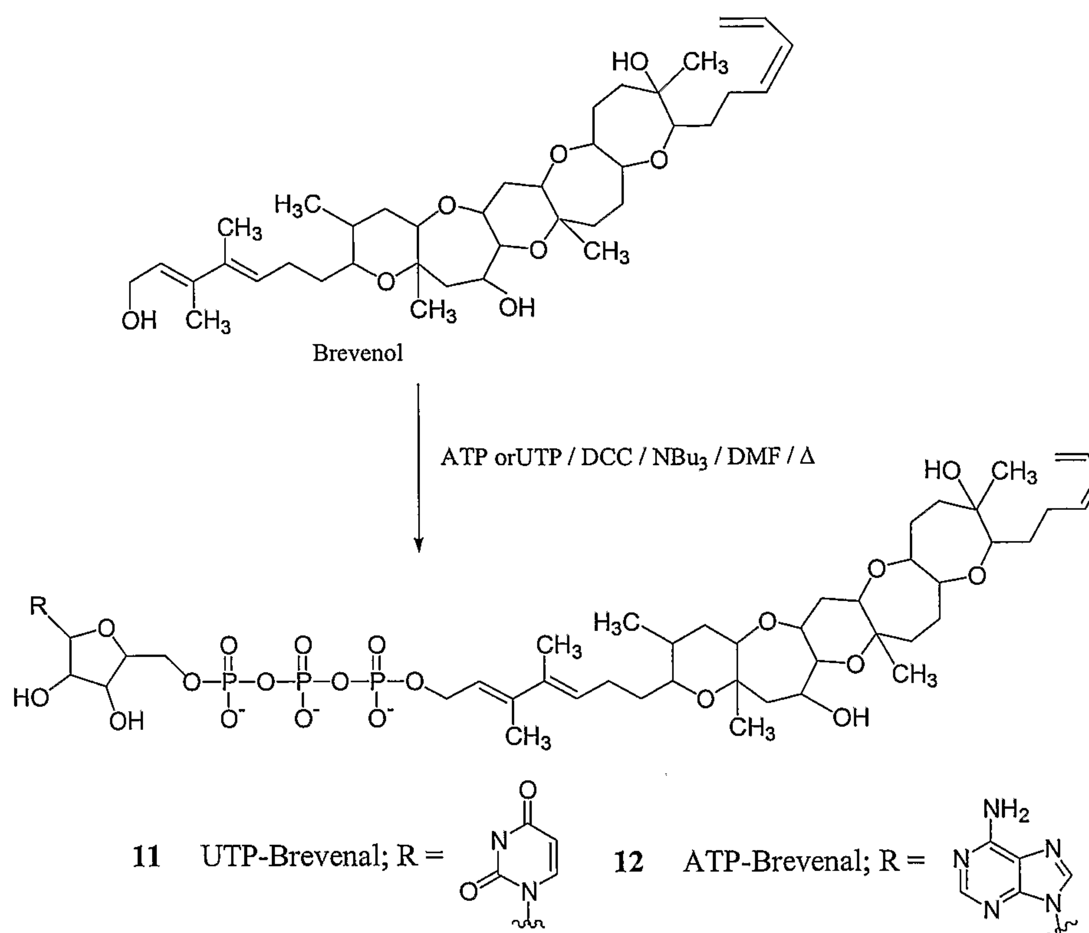
Scheme 7: Synthesis of UTP- and ATP-Brevenal
