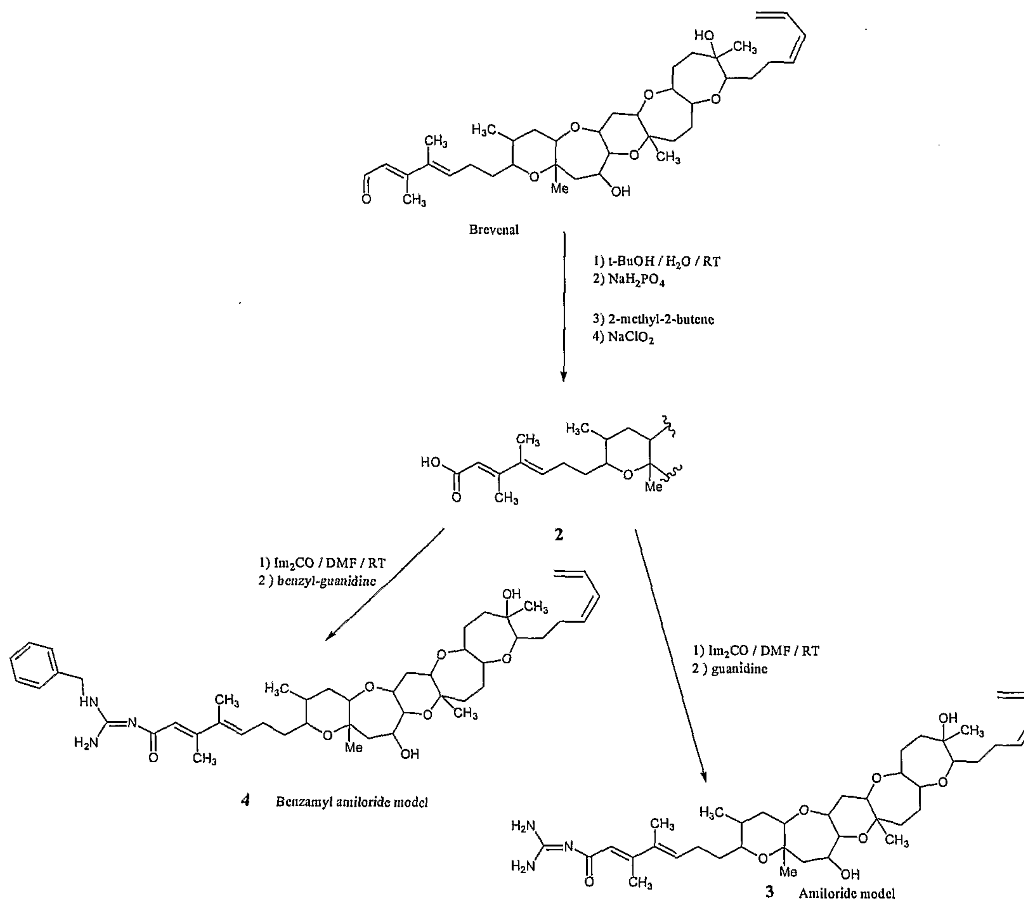
Scheme 2: Guanidine introduction on the \alpha , \beta unsaturated aldehyde sidechain of brevenal
