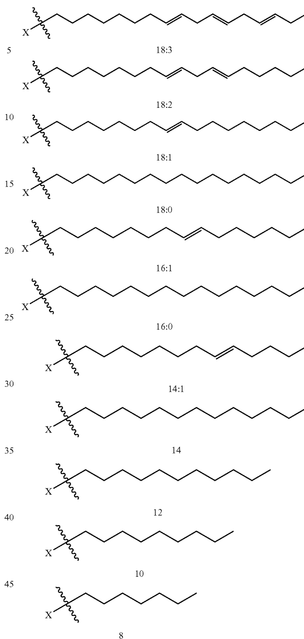
Structure 1A
