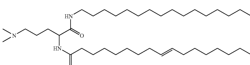
Compound 33
