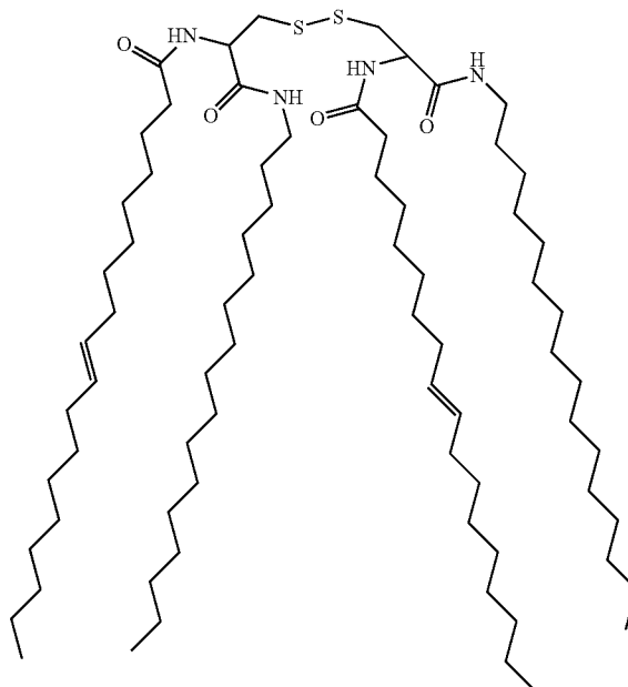
Compound 49
