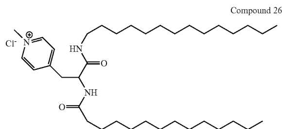
Compound 26
