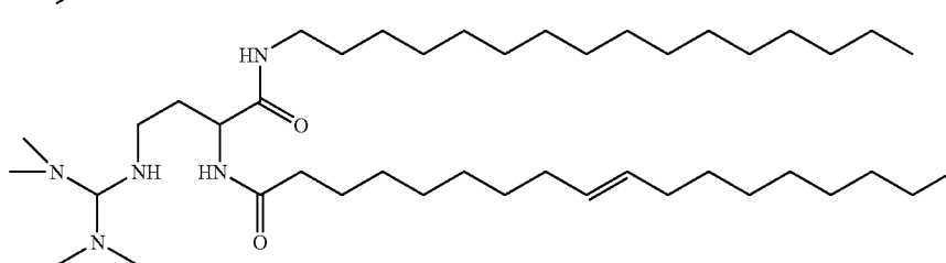
Compound 18
