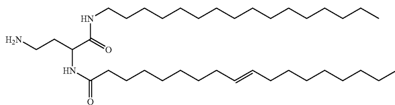
Compound 35
