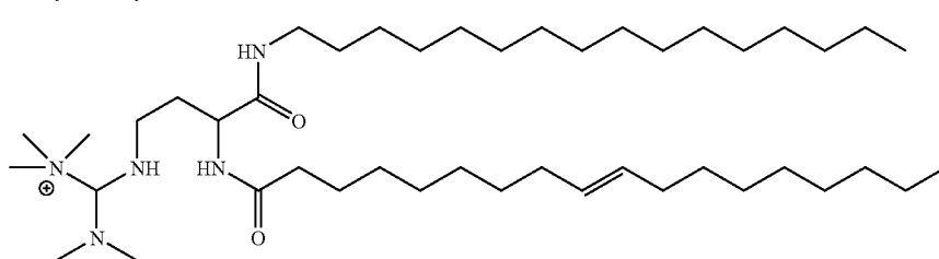
Compound 19
