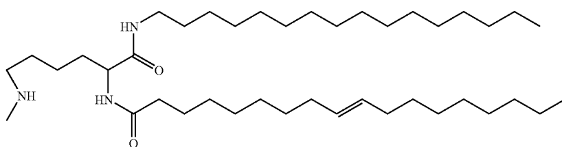
Compound 28
