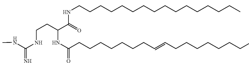
Compound 12
