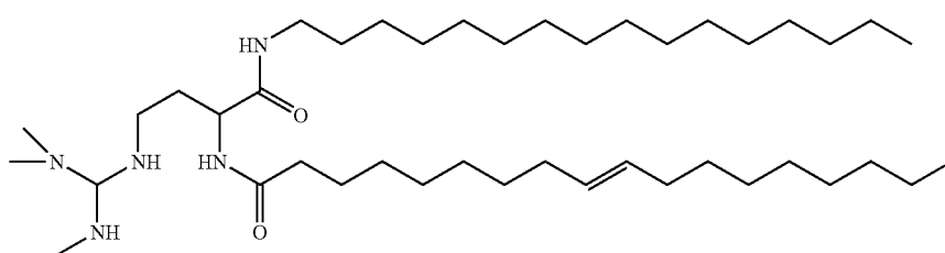
Compound 17
