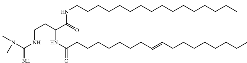
Compound 13
