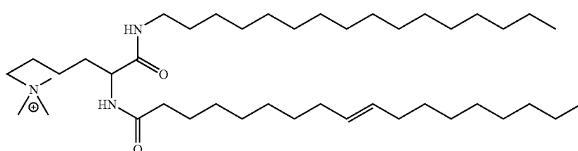
Compound 30
