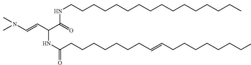
Compound 40
