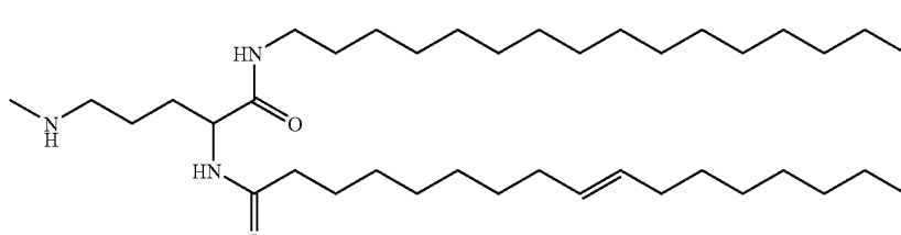
Compound 32
