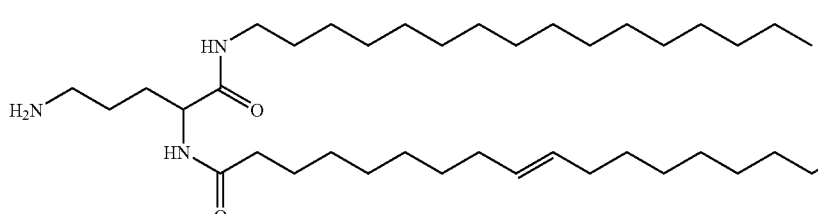
Compound 31
