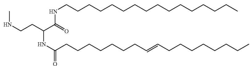
Compound 36
