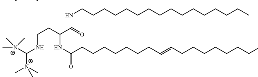
Compound 20
