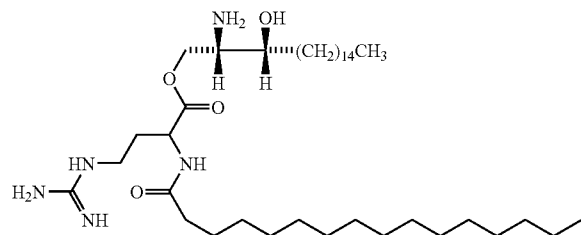
Compound 5 5
