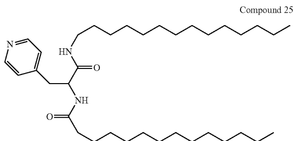
Compound 25
