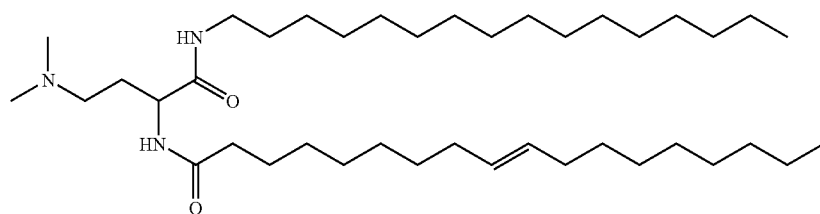
Compound 37
