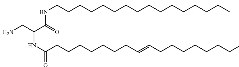
Compound 21
