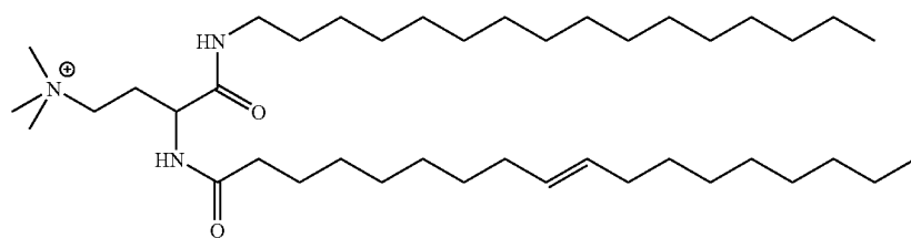
Compound 38
