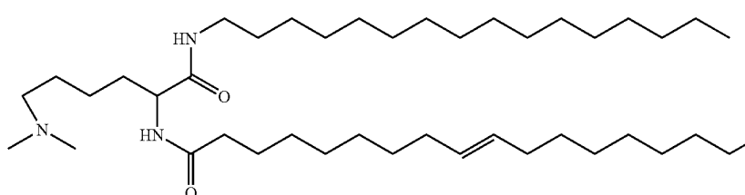
Compound 29
