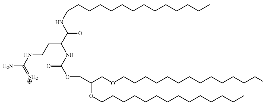
Compound 8
