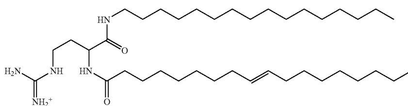
Compound 11
