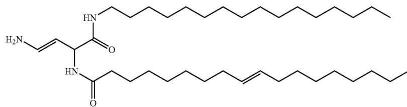
Compound 39
