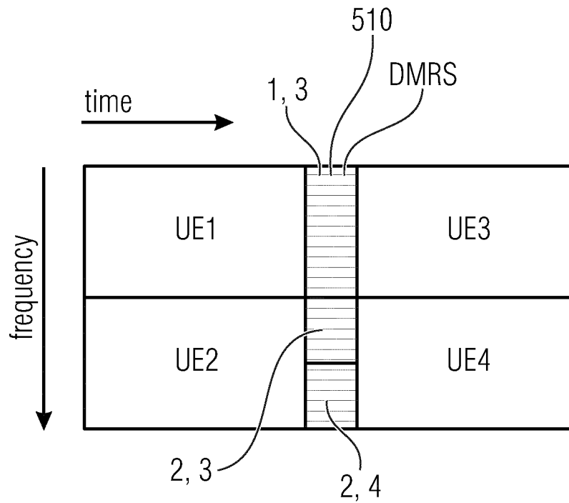
Multiplexing of UEs with different bandwidth allocations
