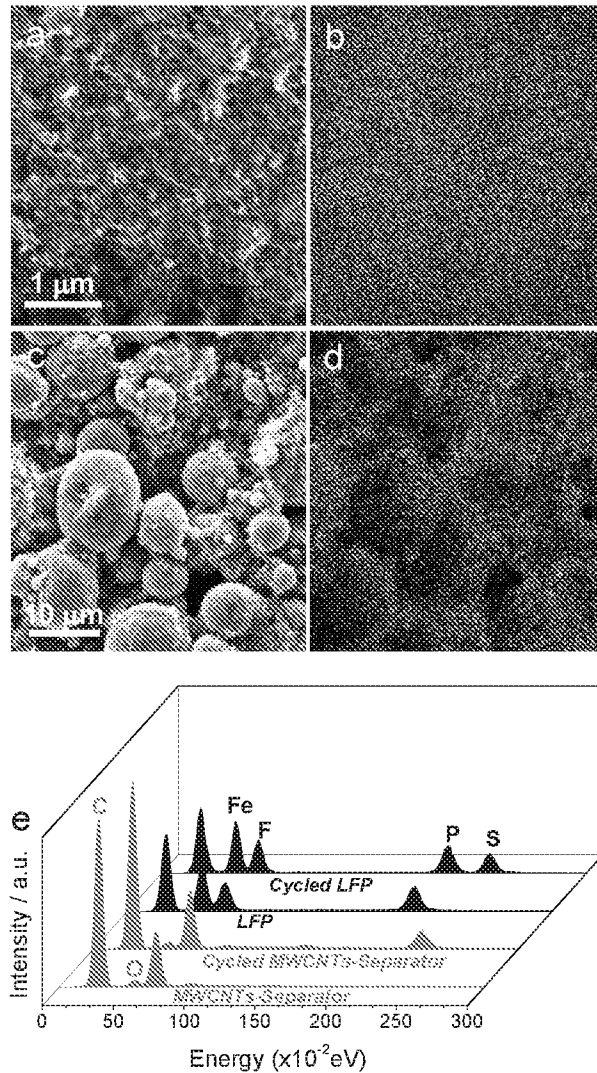
Figure 6. (a) SEM of cyclized MWCNT-separator and relative (b) elemental mapping images. (c) SEM of cyclized LFP cathode and (d) elemental mapping images. The colour of red, yellow, and blue-green represent the distribution of carbon, sulfur and LFP, respectively. (e) Energy-dispersive X-ray spectroscopy of battery using Li 2 S 8 -based electrolyte.
