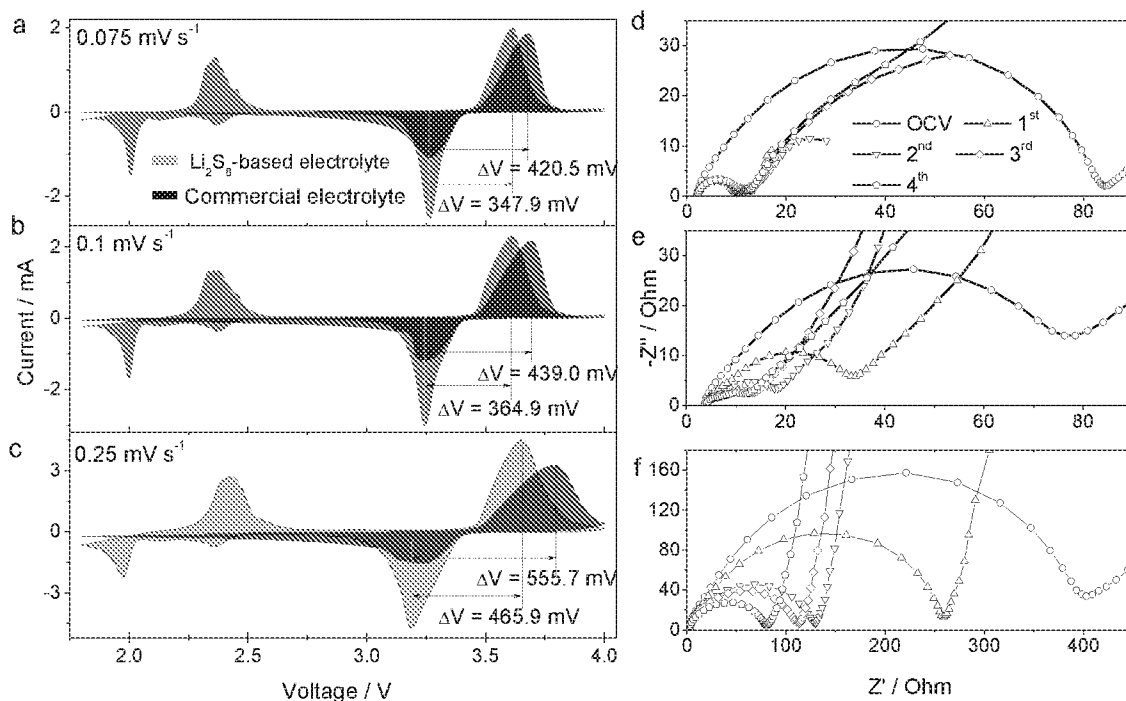
Figure 10. Comparative cyclic voltammetry of LFP lithium battery using \text{Li}_2\text{S}_8 -based electrolyte and commercial electrolyte scanning from (a) 0.075 \text{mV s}^{-1} , (b) 0.1 \text{mV s}^{-1} to (c) 0.25 \text{mV s}^{-1} . Electrochemical impedance spectroscopy of batteries using different electrolyte, (d) electrolyte \text{Li}_2\text{S}_8 -based electrolyte, (e) commercial electrolyte and (f) electrolyte without \text{Li}_2\text{S}_8 as cycling. The polarization of battery using \text{Li}_2\text{S}_8 -based electrolyte are about 347.9 mV, 364.9 mV, and 465.9 mV, significantly lower than 420.5 mV, 439.0 mV and 555.7 mV of commercial LIB battery electrolyte as increasing the scan rate from 0.075-0.25 \text{mV s}^{-1} . Also, the corresponding charge potentials of 3.61 V, 3.61 V and 3.65 V are much lower than 3.68 V, 3.69 V and 3.79 V of commercial LIB battery electrolyte.
