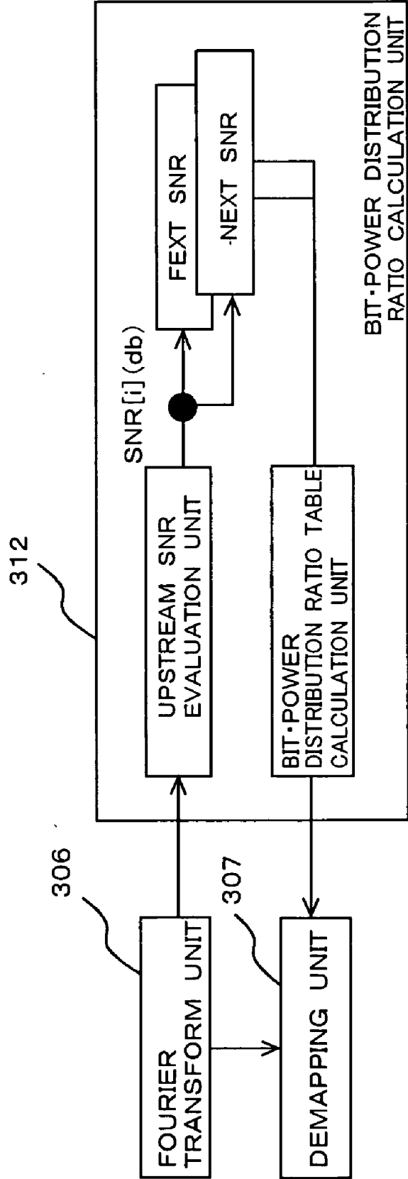
FIG. 5 PRIOR ART
