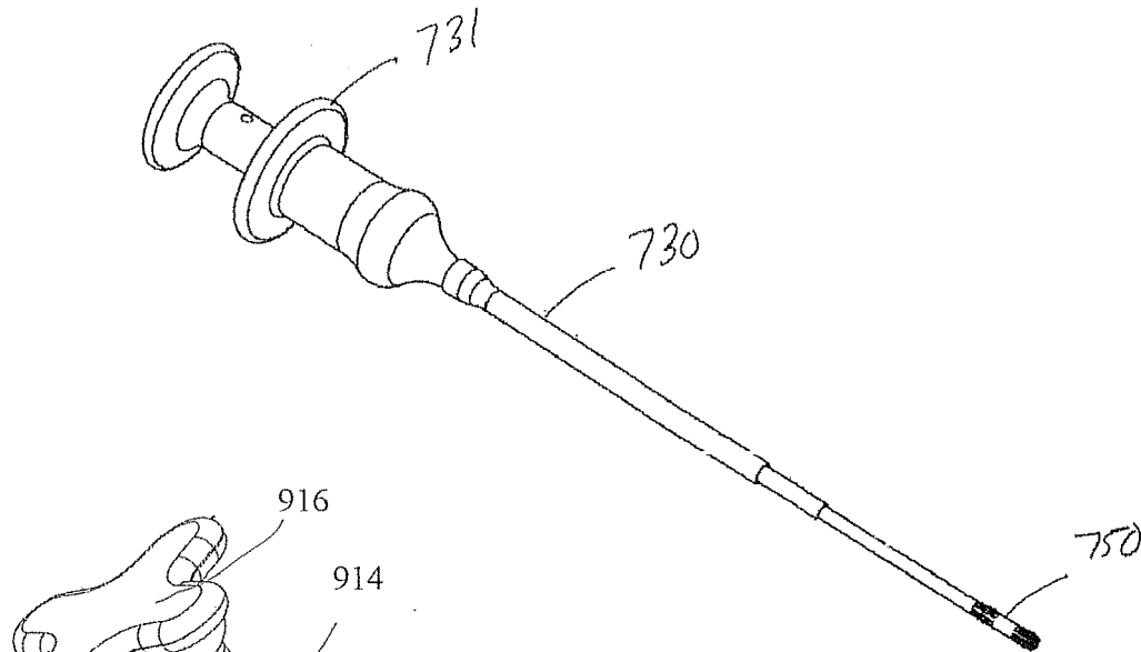
FIG. 10 PRIOR ART
