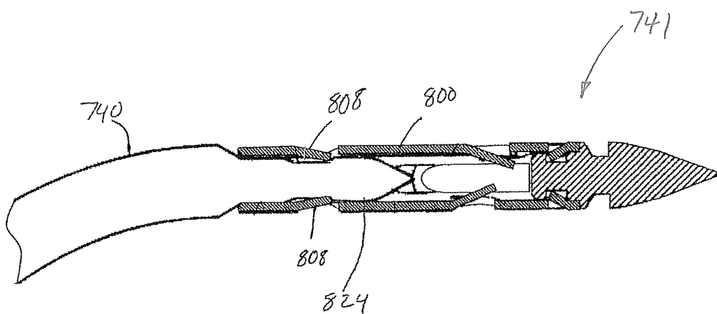
FIG. 9 PRIOR ART
