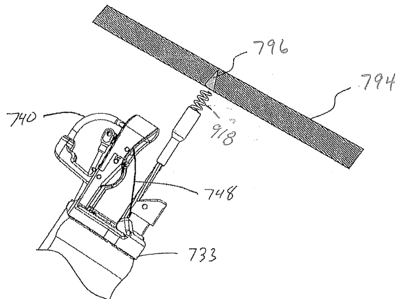
FIG. 13 PRIOR ART
