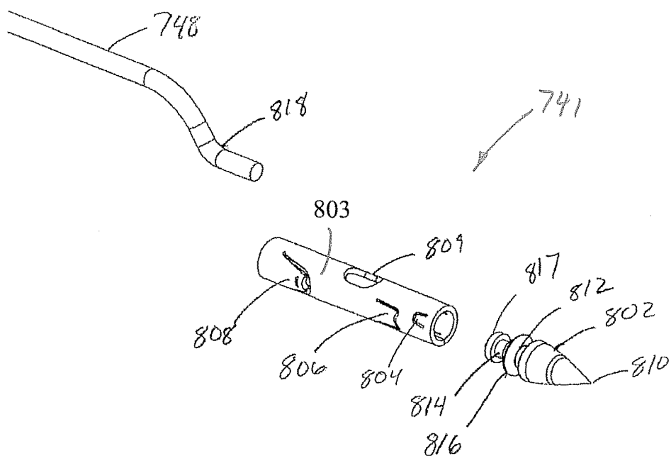
FIG. 7 PRIOR ART
