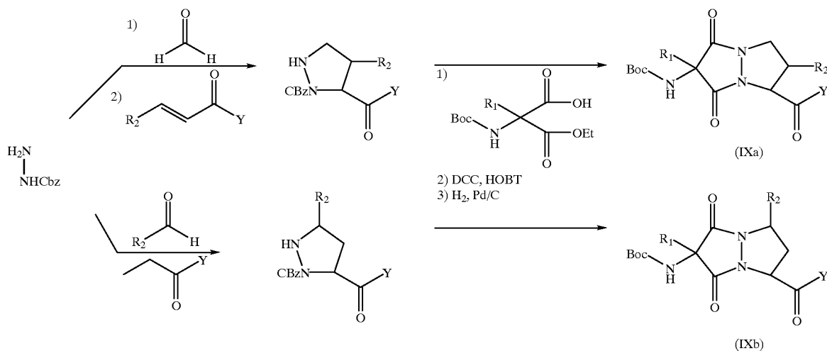
Reaction Scheme (8)
