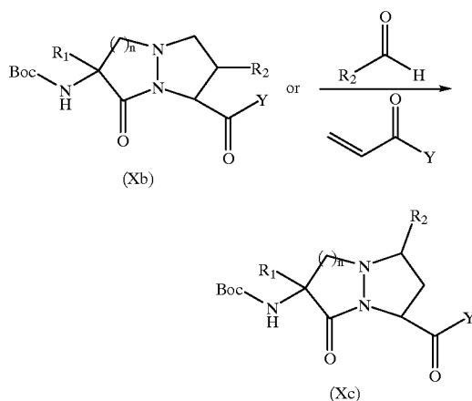
Reaction Scheme (9)
