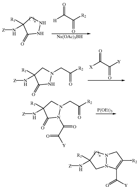
Reaction Scheme (16)
