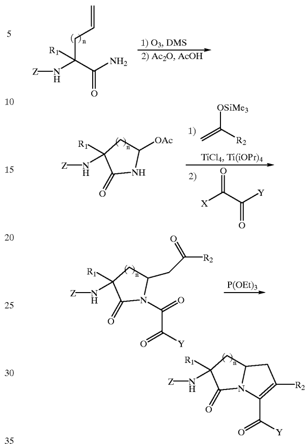
Reaction Scheme (17)
