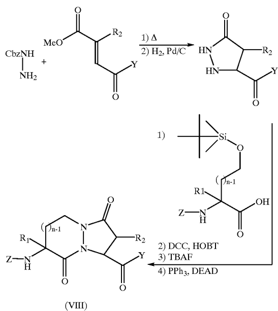
Reaction Scheme (7)
