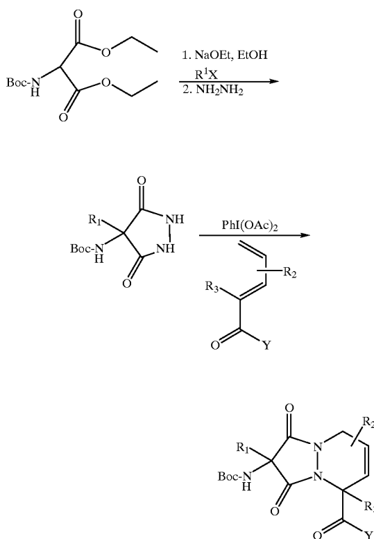
Reaction Scheme (15)
