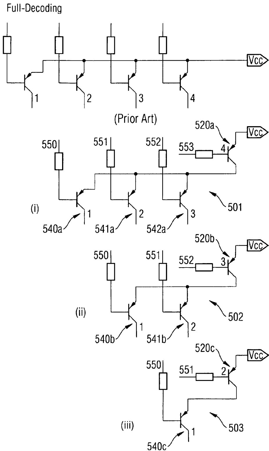
Decoding technique using all the column control input
