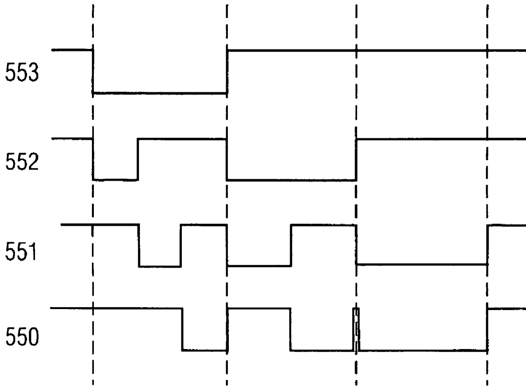
Timing Diagram with full-decoding
