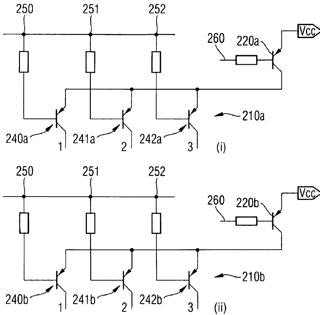
Row Decoding for output lines 1-4
