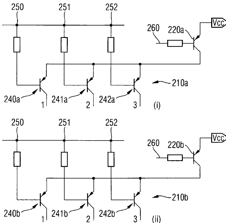
Row Decoding for output lines 1-4
