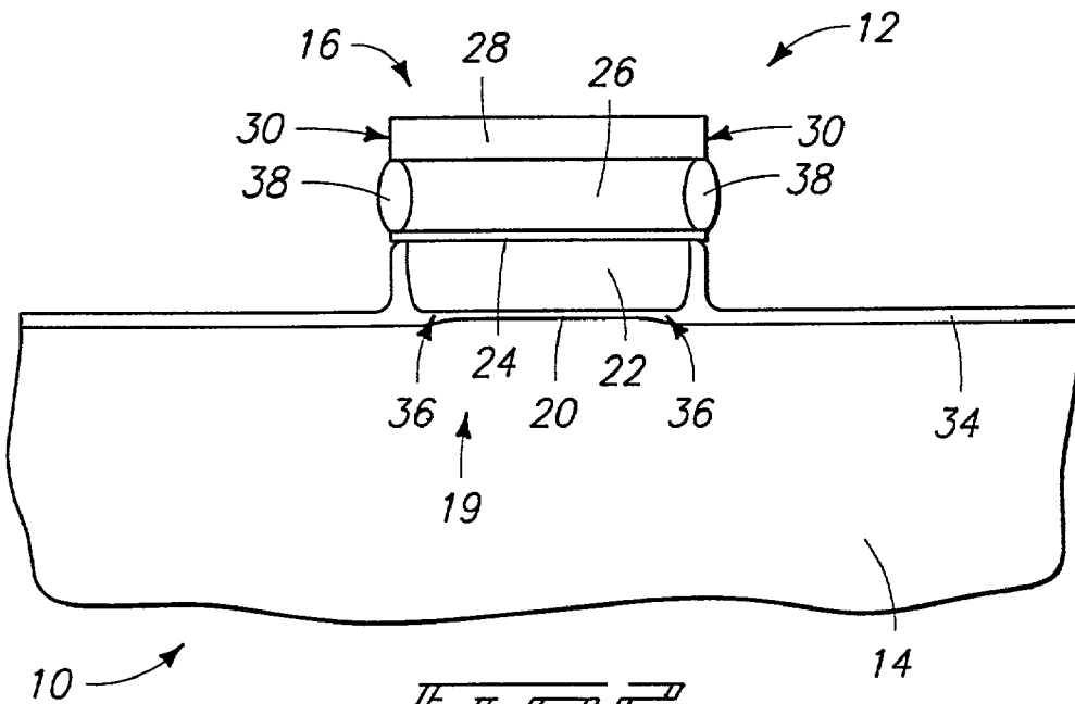
Fig. 2 PRIOR ART
