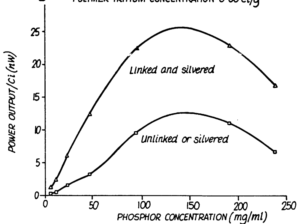
Fig.2. POLYMER TRITIUM CONCENTRATION 6.06 Ci/g
