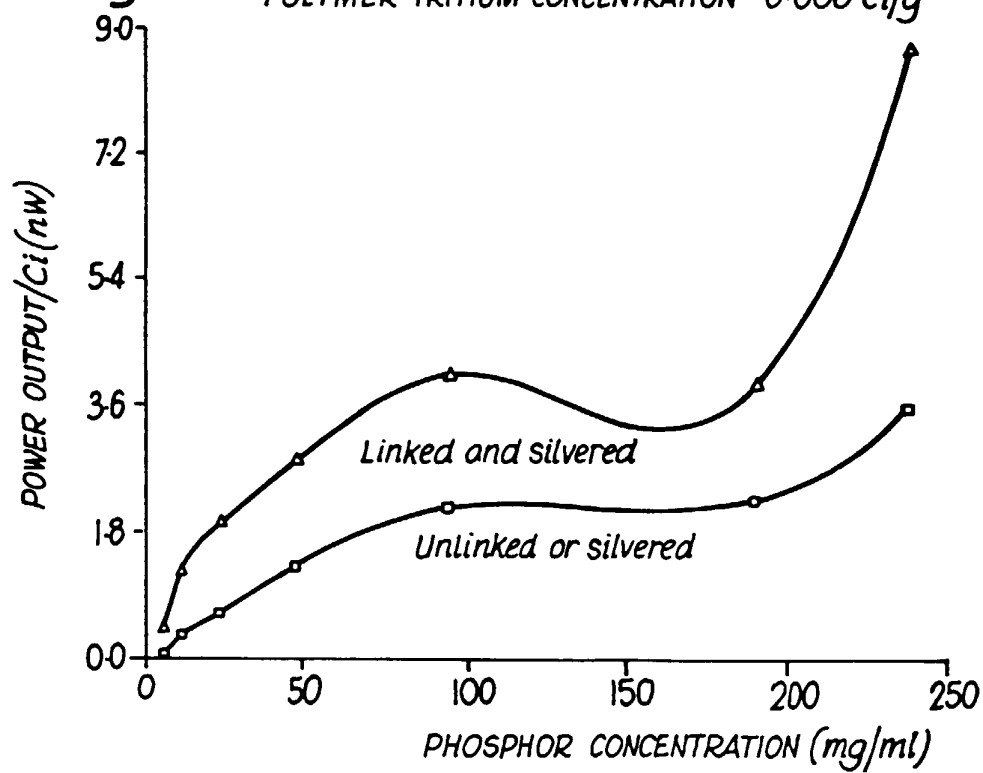
Fig.3. POLYMER TRITIUM CONCENTRATION 0.606 Ci/g
