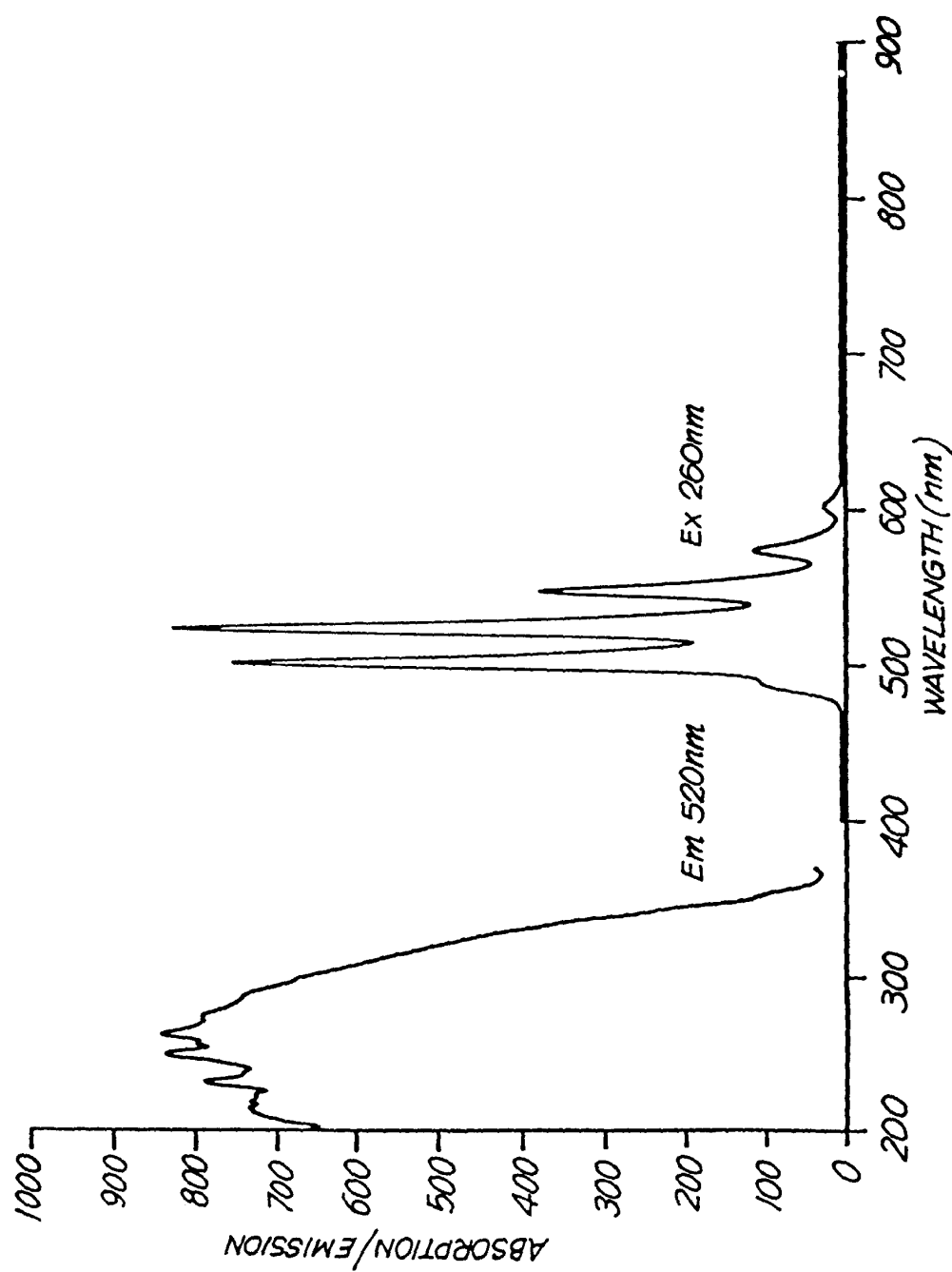
Fig.12 Excitation/Emission Spectra of Bis(imidotetraphenyl)diphosphinic acid)uranium dioxide(II)
