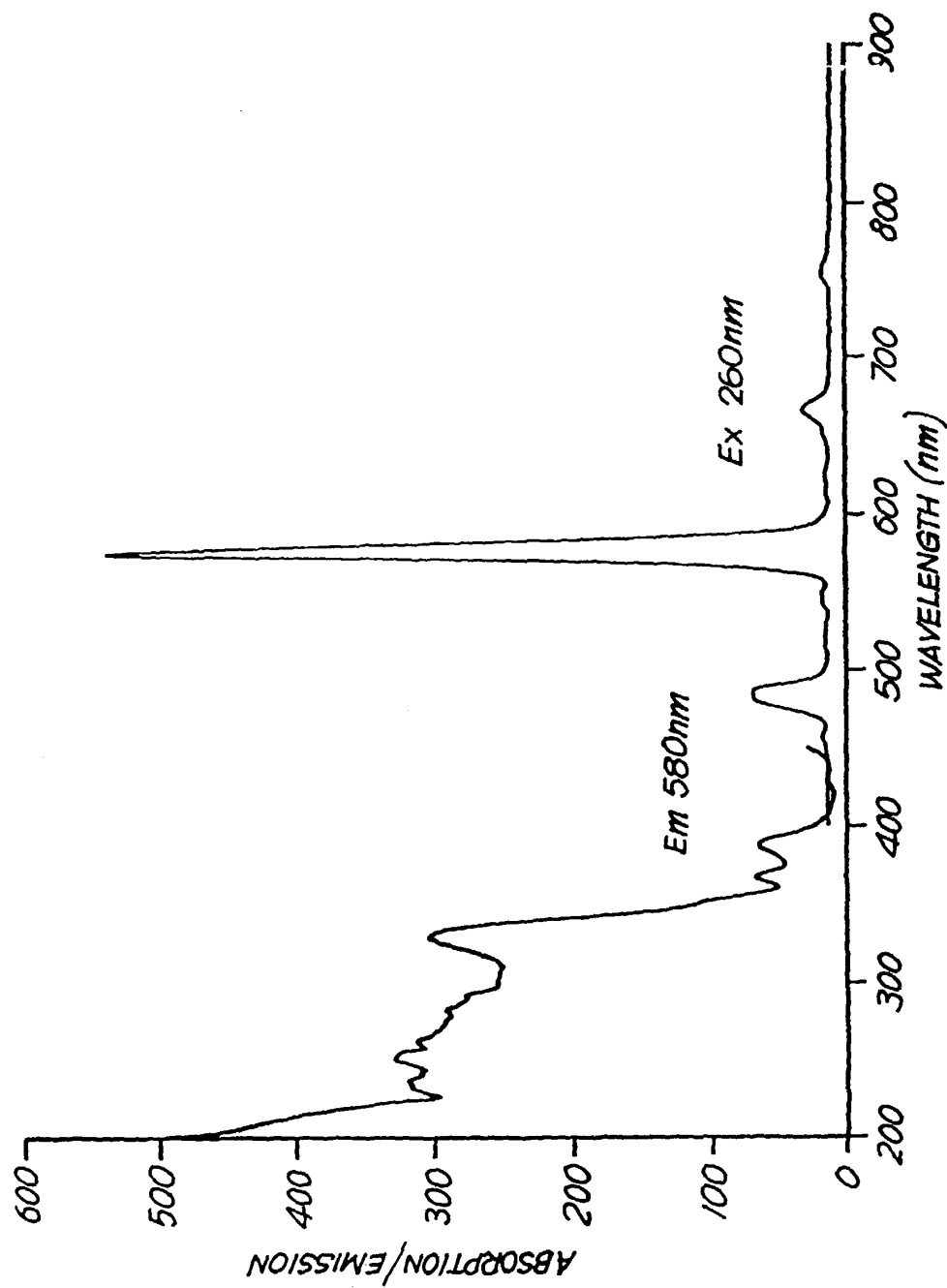
Fig.11 Excitation/Emission Spectra of Tris(2,2,6,6-tetramethyl-3,5-heptanedionato)dysprosium(III) Diphenylphosphonimido triphenylphosphorane
