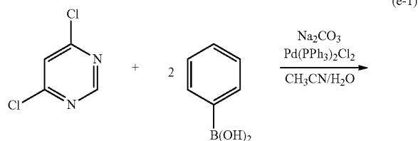
[Chemical Formula 43]
