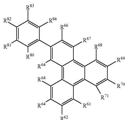
[Chemical Formula 14]
