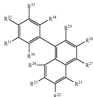
[Chemical Formula 2]
