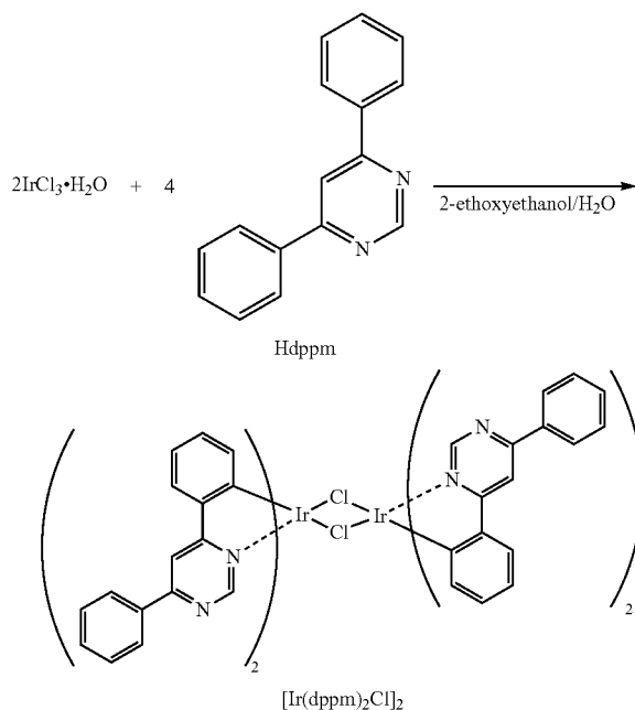
[Chemical Formula 44]
