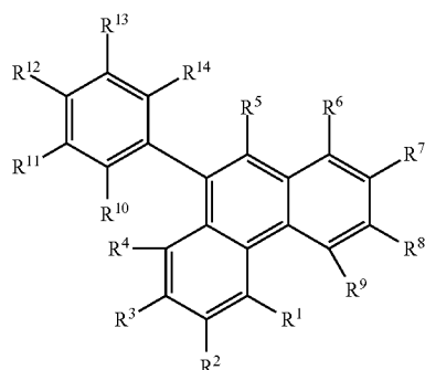
[Chemical Formula 1]
