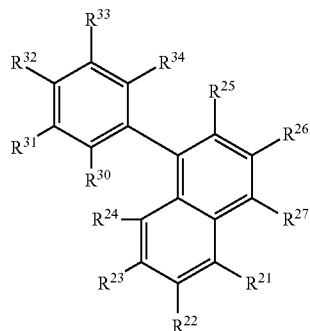
[Chemical Formula 7]
