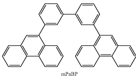
[Chemical Formula 30]
