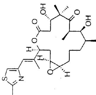
epothilone A
