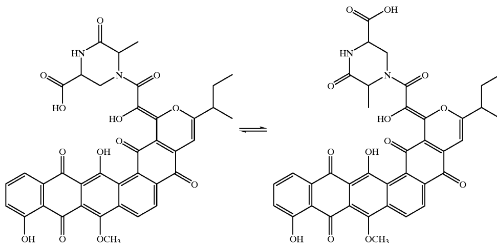
Scheme: Rotameric mixture of bravomicin
