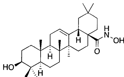
(3β) 3-Hydroxy- N -hydroxy-olean-12-en-28-amide
