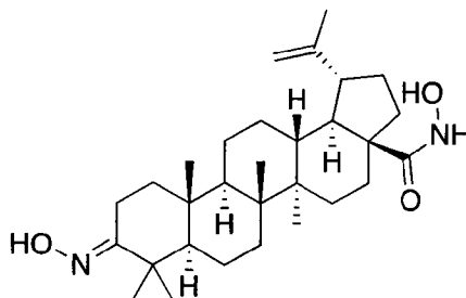
3-Hydroxyimino-N-hydroxy-lup-20(29)-en-28-amide
