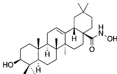
(3β) 3-Hydroxy-N-hydroxy-olean-12-en-28-amide
