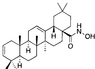
Oleana-2,12-dien- N -hydroxy-28-amide
