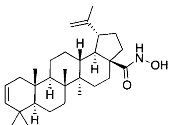
Lupa-2,20(29)-dien-N-hydroxy-28-amide
