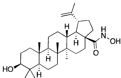
(3β) 3-Hydroxy-N-hydroxy-lup-20(29)-en-28-amide
