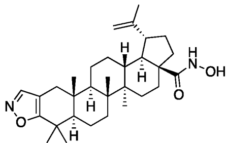
Lup-2-eno[2,3-d]isoxazol- N -hydroxy-28-amide
