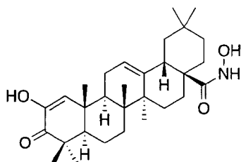
2-Hydroxy-3-oxo-oleana-1,12-dien-N-hydroxy-28-amide.
