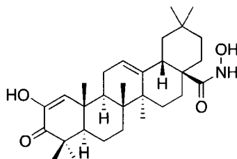
2-Hydroxy-3-oxo-oleana-1,12-dien-N-hydroxy-28-amide.
