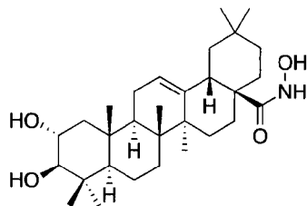
(2 \alpha ,3 \beta ) 2,3-Dihydroxy-N-hydroxy-olean-12-en-28-amide
