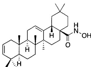
Oleana-2,12-dien-N-hydroxy-28-amide
