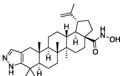
1' H -Lup-20(29)-eno[3,2- c ]pyrazol- N -hydroxy-28-amide
