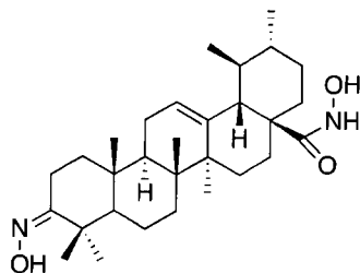
3 Hydroxyimino- N -hydroxy-urs-12-en-28-amide
