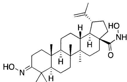
3-Hydroxyimino- N -hydroxy-lup-20(29)-en-28-amide
