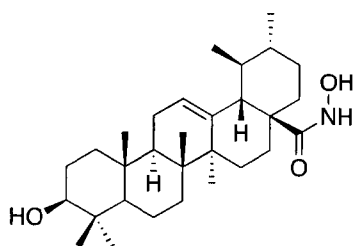
(3 \beta ) 3-Hydroxy- N -hydroxy-urs-12-en-28-amide
