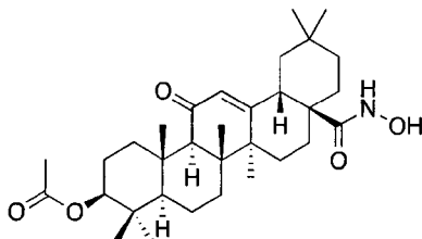
(3β) 3-Acetyloxy-11-oxo-olean-12-en-N-hydroxy-28-amide
