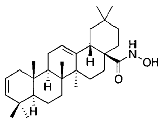
Oleana-2,12-dien- N -hydroxy-28-amide
