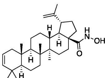
Lupa-2,20(29)-dien-N-hydroxy-28-amide
