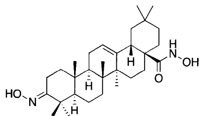
3-Hydroxyimino- N -hydroxy-olean-12-en-28-amide
