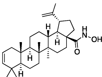
Lupa-2,20(29)-dien- N -hydroxy-28-amide
