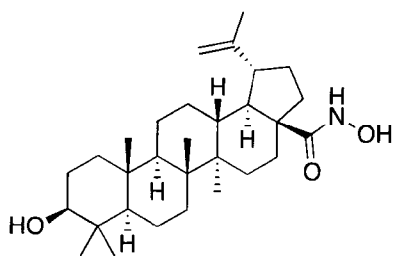
(3β) 3-Hydroxy-N-hydroxy-lup-20(29)-en-28-amide
