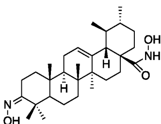
3-Hydroxyimino- N -hydroxy-urs-12-en-28-amide
