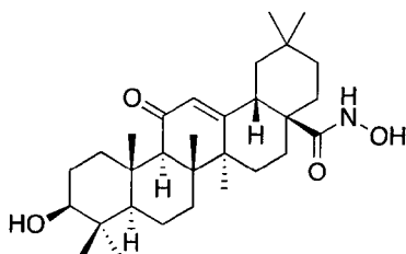
(3 \beta ) 3-Hydroxy-11-oxo-olean-12-en- N -hydroxy-28-amide
