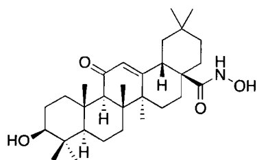
(3β)-3-Hydroxy-11-oxo-olean-12-en- N -hydroxy-28-amide
