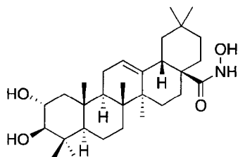
(2α,3β) 2,3-Dihydroxy-N-hydroxy-olean-12-en-28-amide
