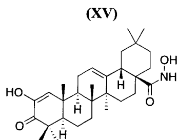
2-Hydroxy-3-oxo-oleana-1,12-dien-N-hydroxy-28-amide.
