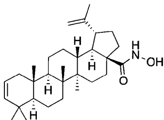
Lupa-2,20(29)-dien-N-hydroxy-28-amide
