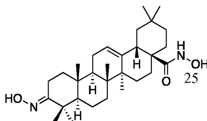
3-Hydroxyimino- N -hydroxy-olean-12-en-28-amide
