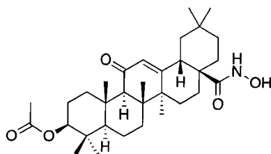
(3β)-3-Acetyloxy-11-oxo-olean-12-en- N -hydroxy-28-amide
