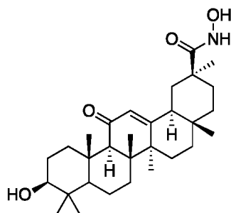
(3 \beta )-3-Hydroxy-11-oxo-olean-12-en-N-hydroxy-29-amide
