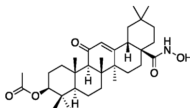
(3β) 3-Acetyloxy-11-oxo-olean-12-en-N-hydroxy-28-amide;
