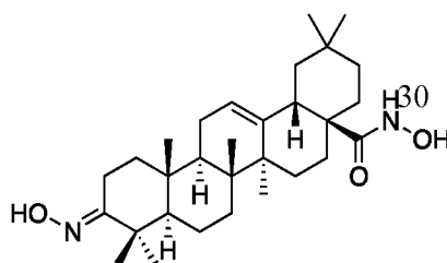
3-Hydroxyimino-N-hydroxy-olean-12-en-28-amide
