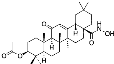
(3 \beta ) 3-Acetyloxy-11-oxo-olean-12-en- N -hydroxy-28-amide
