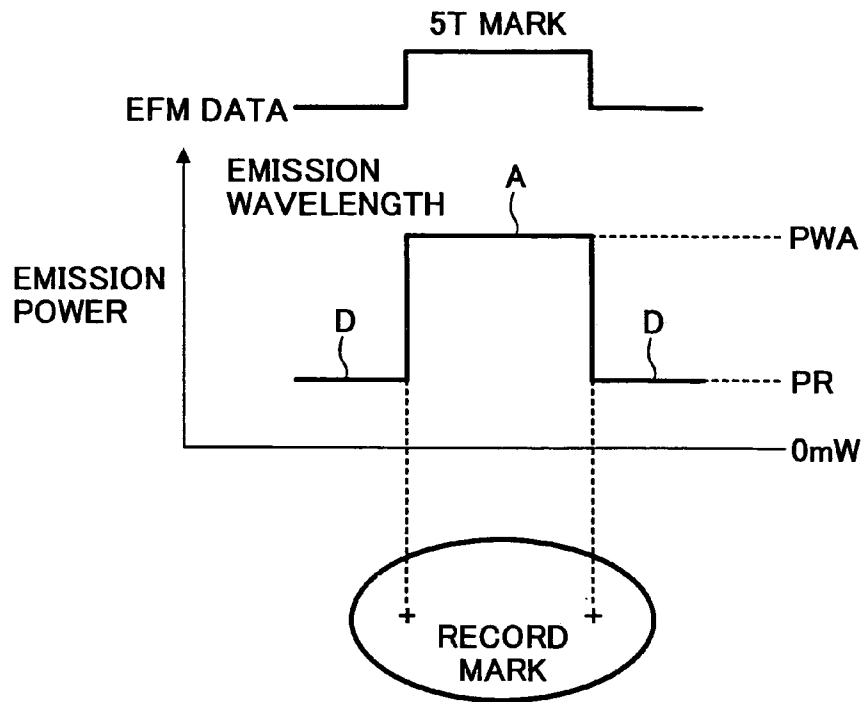
FIG. 17 BACKGROUND ART
