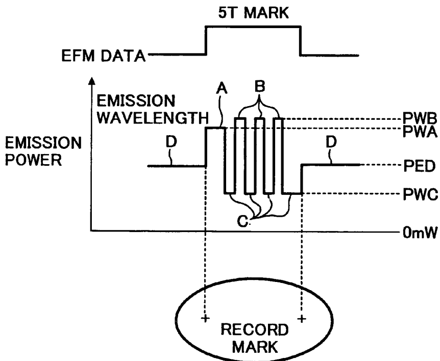
FIG. 18 BACKGROUND ART
