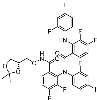
Dimer Acetonide Exact Mass: 897.35 (c)
