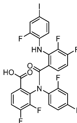
PD-0315209 Dimer Exact Mass: 767.88 (b)
