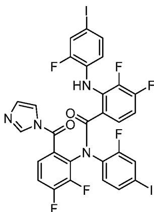
Dimer Imidazolid Exact Mass: 817.91 (a)
