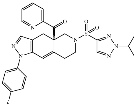
11CT (R)-(1-(4-fluorophenyl)-6-((2-isopropyl-2H-1,2,3-triazol-4-yl)sulfonyl)-4,4a,5,6,7,8-hexahydro-1H-pyrazolo[3,4-g]isoquinolin-4a-yl)(pyridin-2-yl)methanone
