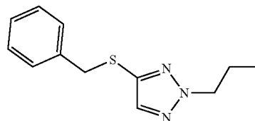
87a 4-(benzylthio)-2-propyl-2H-1,2,3-triazole
