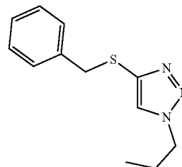
87c 4-(benzylthio)-1-propyl-1H-1,2,3-triazole
