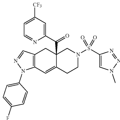
11CG (R)-(1-(4-fluorophenyl)-6-((1-methyl-1H-1,2,3-triazol-4-yl)sulfonyl)-4,4a,5,6,7,8-hexahydro-1H-pyrazolo[3,4-g]isoquinolin-4a-yl)(4-(trifluoromethyl)pyridin-2-yl)methanone
