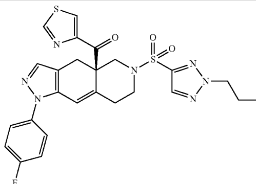
11CQ (R)-(1-(4-fluorophenyl)-6-((2-propyl-2H-1,2,3-triazol-4-yl)sulfonyl)-4,4a,5,6,7,8-hexahydro-1H-pyrazolo[3,4-g]isoquinolin-4a-yl)(thiazol-4-yl)methanone
