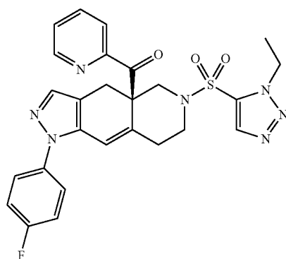
11CI (R)-(6-((1-ethyl-1H-1,2,3-triazol-5-yl)sulfonyl)-1-(4-fluorophenyl)-4,4a,5,6,7,8-hexahydro-1H-pyrazolo[3,4-g]isoquinolin-4a-yl)(pyridin-2-yl)methanone
