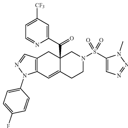
11CF (R)-(1-(4-fluorophenyl)-6-((1-methyl-1H-1,2,3-triazol-5-yl)sulfonyl)-4,4a,5,6,7,8-hexahydro-1H-pyrazolo[3,4-g]isoquinolin-4a-yl)(4-(trifluoromethyl)pyridin-2-yl)methanone
