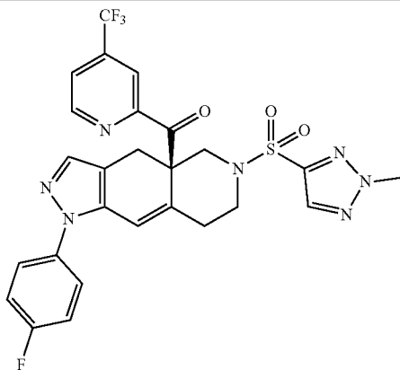
11CE (R)-(1-(4-fluorophenyl)-6-((2-methyl-2H-1,2,3-triazol-4-yl)sulfonyl)-4,4a,5,6,7,8-hexahydro-1H-pyrazolo[3,4-g]isoquinolin-4a-yl)(4-(trifluoromethyl)pyridin-2-yl)methanone
