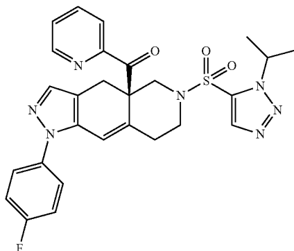
11CU (R)-(1-(4-fluorophenyl)-6-((1-isopropyl-1H-1,2,3-triazol-5-yl)sulfonyl)-4,4a,5,6,7,8-hexahydro-1H-pyrazolo[3,4-g]isoquinolin-4a-yl)(pyridin-2-yl)methanone
