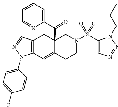
11CO (R)-(1-(4-fluorophenyl)-6-((1-propyl-1H-1,2,3-triazol-5-yl)sulfonyl)-4,4a,5,6,7,8-hexahydro-1H-pyrazolo[3,4-g]isoquinolin-4a-yl)(pyridin-2-yl)methanone
