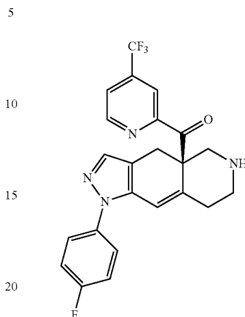
Intermediate 78. (R)-(1-(4-fluorophenyl)-4,4a,5,6,7,8-hexahydro-1H-pyrazolo[3,4-g]isoquinolin-4a-yl)(4-(trifluoromethyl)pyridin-2-yl)methanone
