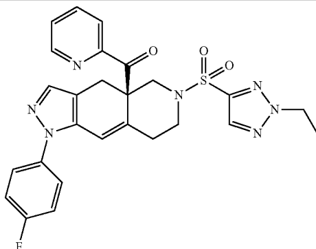
11CH (R)-(6-((2-ethyl-2H-1,2,3-triazol-4-yl)sulfonyl)-1-(4-fluorophenyl)-4,4a,5,6,7,8-hexahydro-1H-pyrazolo[3,4-g]isoquinolin-4a-yl)(pyridin-2-yl)methanone
