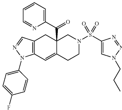
11CP (R)-(1-(4-fluorophenyl)-6-((1-propyl-1H-1,2,3-triazol-4-yl)sulfonyl)-4,4a,5,6,7,8-hexahydro-1H-pyrazolo[3,4-g]isoquinolin-4a-yl)(pyridin-2-yl)methanone
