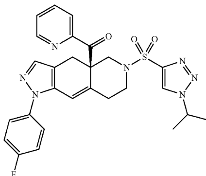
11CV (R)-(1-(4-fluorophenyl)-6-((1-isopropyl-1H-1,2,3-triazol-4-yl)sulfonyl)-4,4a,5,6,7,8-hexahydro-1H-pyrazolo[3,4-g]isoquinolin-4a-yl)(pyridin-2-yl)methanone
