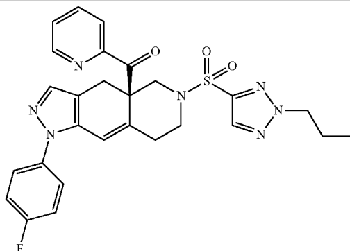
11CN (R)-(1-(4-fluorophenyl)-6-((2-propyl-2H-1,2,3-triazol-4-yl)sulfonyl)-4,4a,5,6,7,8-hexahydro-1H-pyrazolo[3,4-g]isoquinolin-4a-yl)(pyridin-2-yl)methanone
