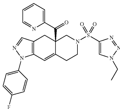
11CJ (R)-(6-((1-ethyl-1H-1,2,3-triazol-4-yl)sulfonyl)-1-(4-fluorophenyl)-4,4a,5,6,7,8-hexahydro-1H-pyrazolo[3,4-g]isoquinolin-4a-yl)(pyridin-2-yl)methanone
