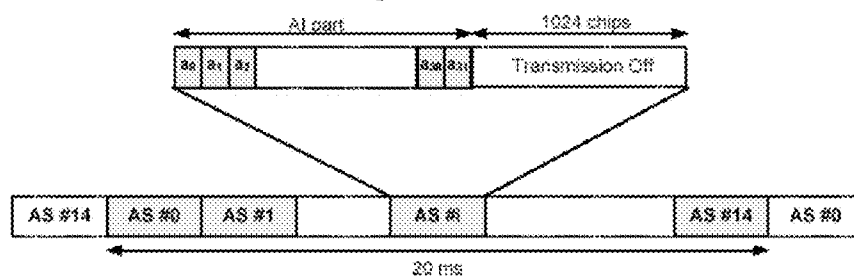
Figure 84: Structure of the AI part
