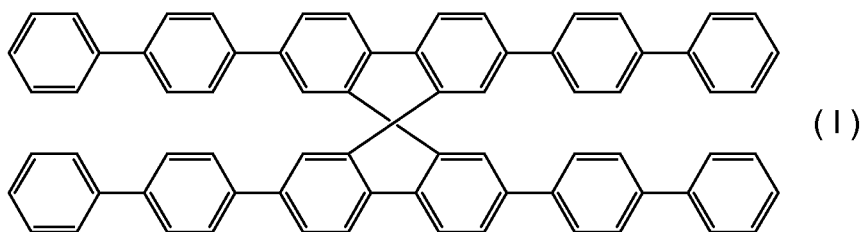
[Chemical Formula 1]
