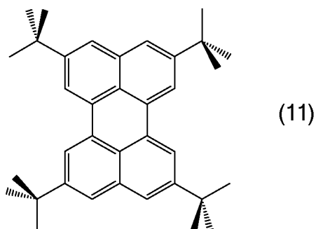
[Chemical Formula 13]
