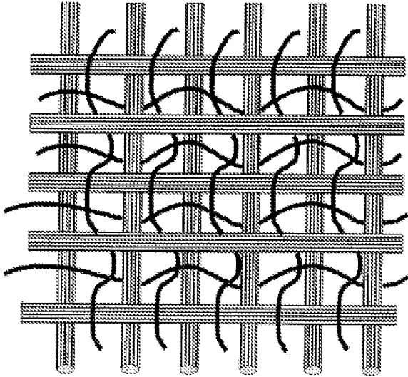
FIG. 1 (PRIOR ART)
