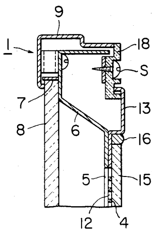
FIG. 1 PRIOR ART
